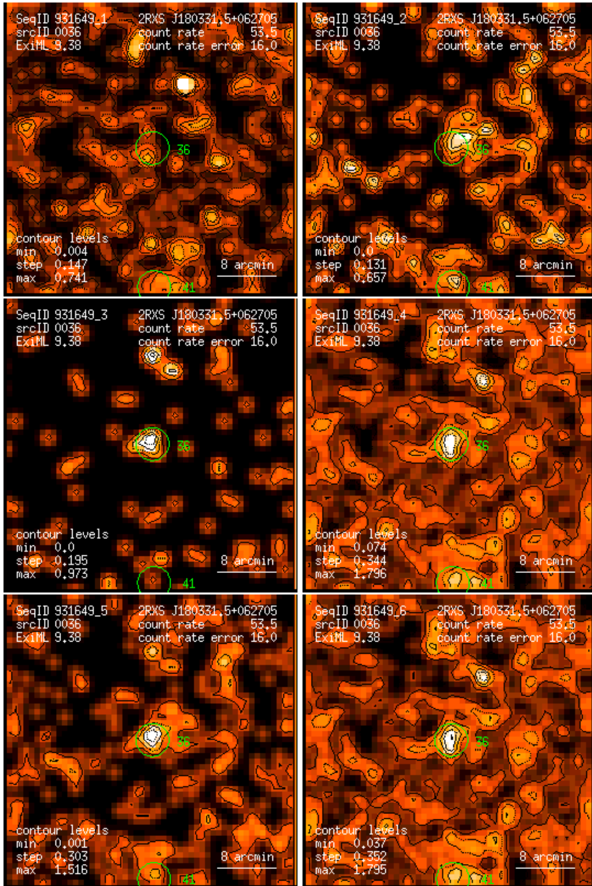
Figure 36: RASS 931649: detection 0036: band rate images, Gaussian filter: (1) PSPC channels 11 – 41, (2) 52 – 90, (3) 91 – 201, (4) 11 – 235, (5) 52 – 201, (6) 11 – 201. Broad band rates in counts/ks. Band rate contour levels in counts/ks/arcmin 2 .
