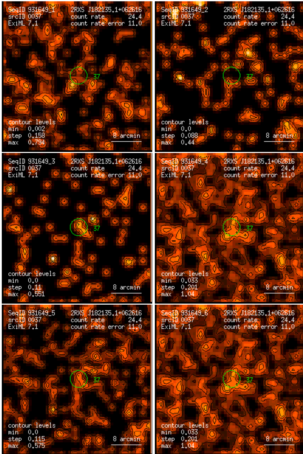
Figure 37: RASS 931649: detection 0037: band rate images, Gaussian filter: (1) PSPC channels 11 – 41, (2) 52 – 90, (3) 91 – 201, (4) 11 – 235, (5) 52 – 201, (6) 11 – 201. Broad band rates in counts/ks. Band rate contour levels in counts/ks/arcmin 2 .
