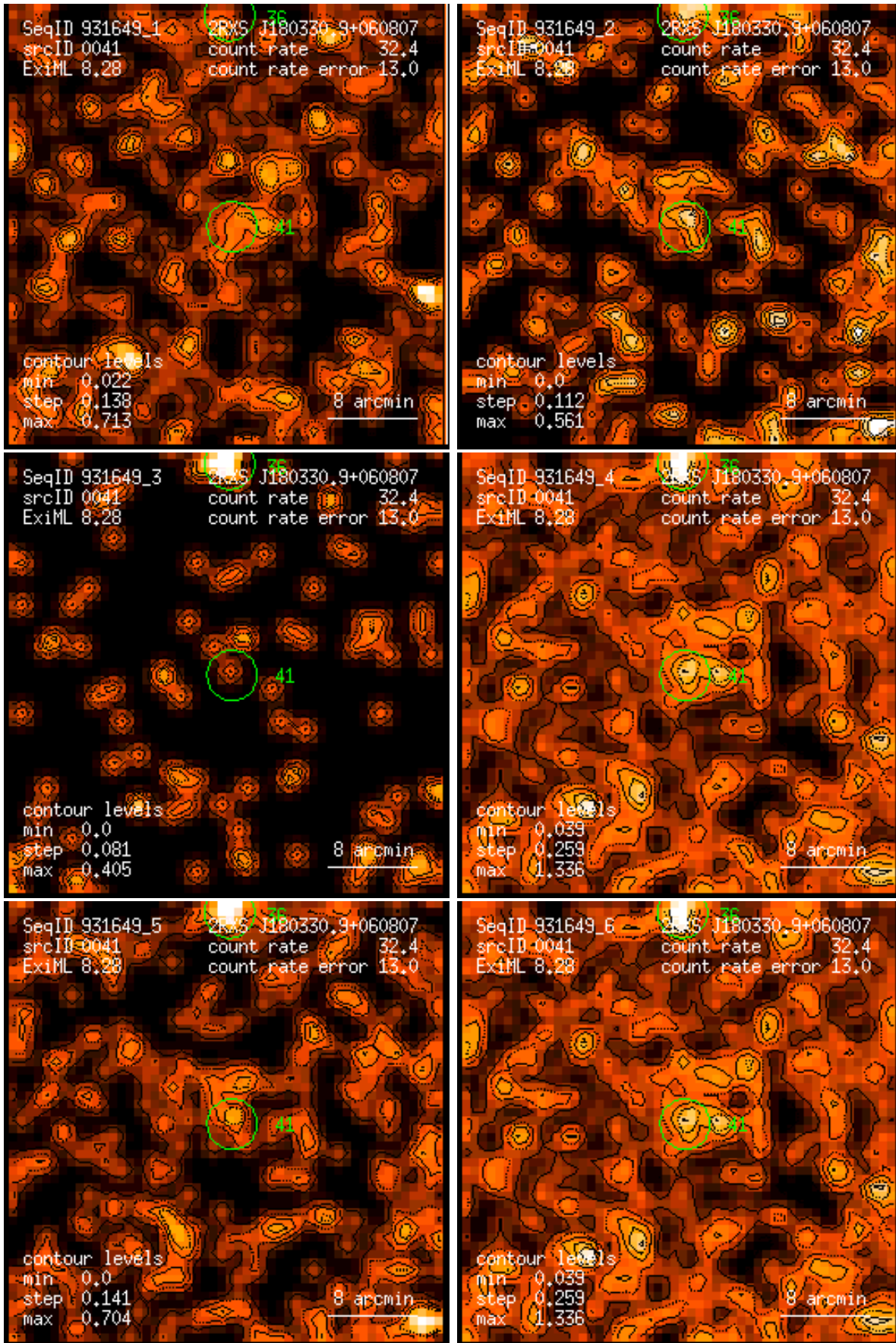
Figure 41: RASS 931649: detection 0041: band rate images, Gaussian filter: (1) PSPC channels 11 – 41, (2) 52 – 90, (3) 91 – 201, (4) 11 – 235, (5) 52 – 201, (6) 11 – 201. Broad band rates in counts/ks. Band rate contour levels in counts/ks/arcmin 2 .
