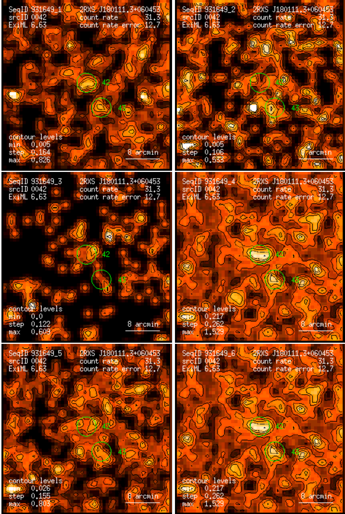
Figure 42: RASS 931649: detection 0042: band rate images, Gaussian filter: (1) PSPC channels 11 – 41, (2) 52 – 90, (3) 91 – 201, (4) 11 – 235, (5) 52 – 201, (6) 11 – 201. Broad band rates in counts/ks. Band rate contour levels in counts/ks/arcmin 2 .
