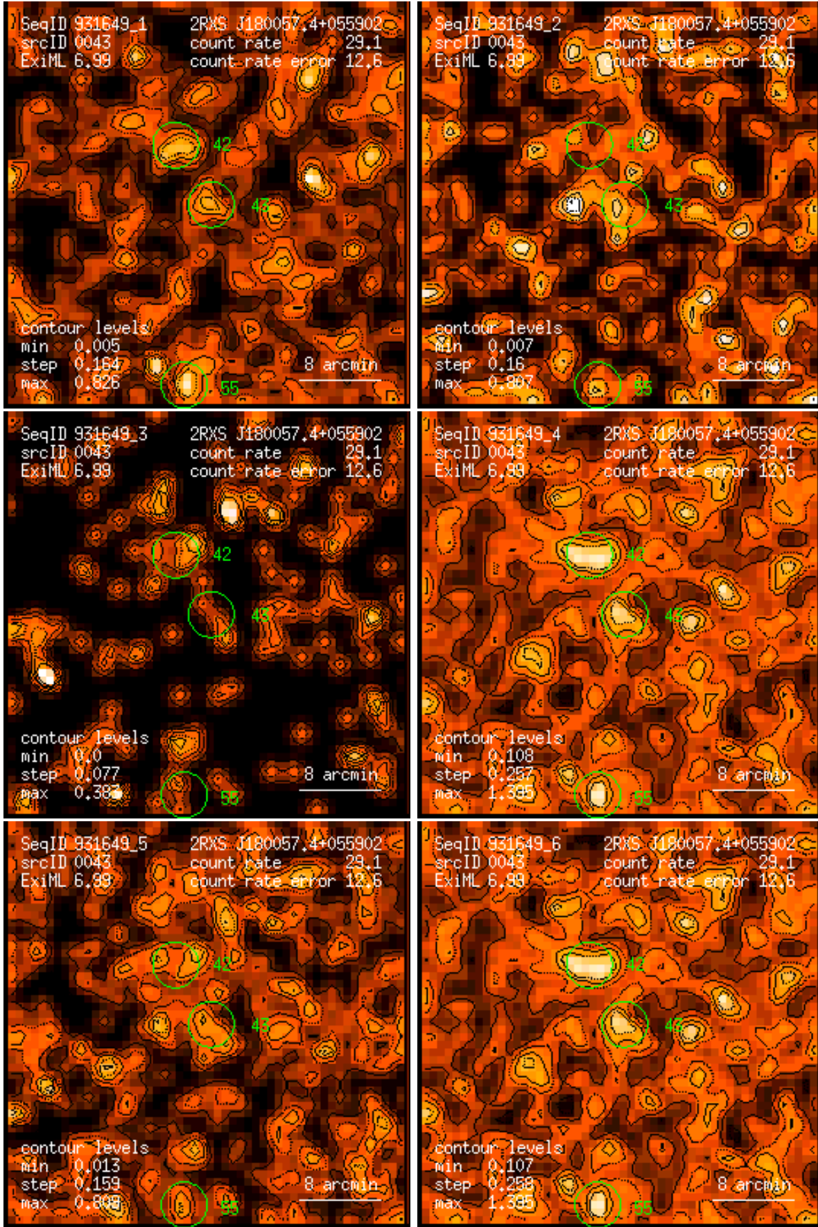
Figure 43: RASS 931649: detection 0043: band rate images, Gaussian filter: (1) PSPC channels 11 – 41, (2) 52 – 90, (3) 91 – 201, (4) 11 – 235, (5) 52 – 201, (6) 11 – 201. Broad band rates in counts/ks. Band rate contour levels in counts/ks/arcmin 2 .
