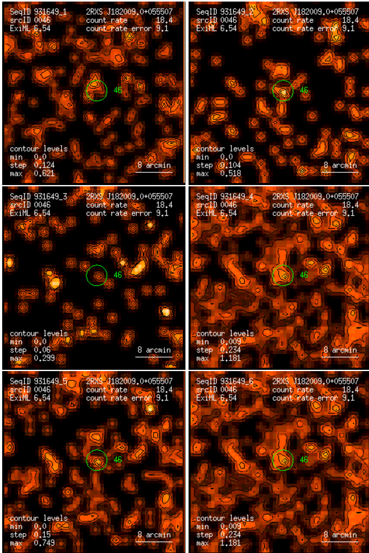
Figure 46: RASS 931649: detection 0046: band rate images, Gaussian filter: (1) PSPC channels 11 – 41, (2) 52 – 90, (3) 91 – 201, (4) 11 – 235, (5) 52 – 201, (6) 11 – 201. Broad band rates in counts/ks. Band rate contour levels in counts/ks/arcmin 2 .
