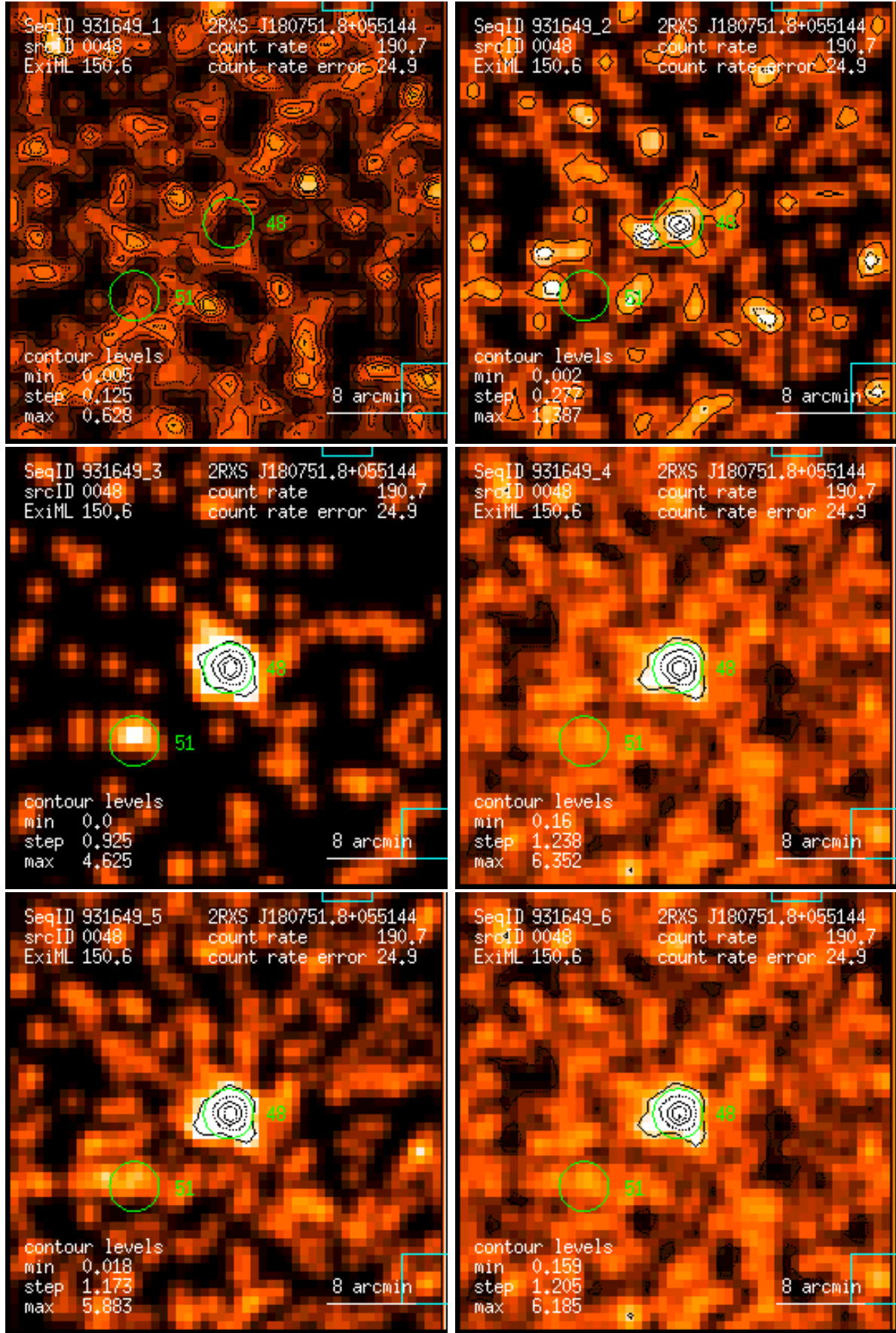
Figure 48: RASS 931649: detection 0048: band rate images, Gaussian filter: (1) PSPC channels 11 – 41, (2) 52 – 90, (3) 91 – 201, (4) 11 – 235, (5) 52 – 201, (6) 11 – 201. Broad band rates in counts/ks. Band rate contour levels in counts/ks/arcmin 2 .
