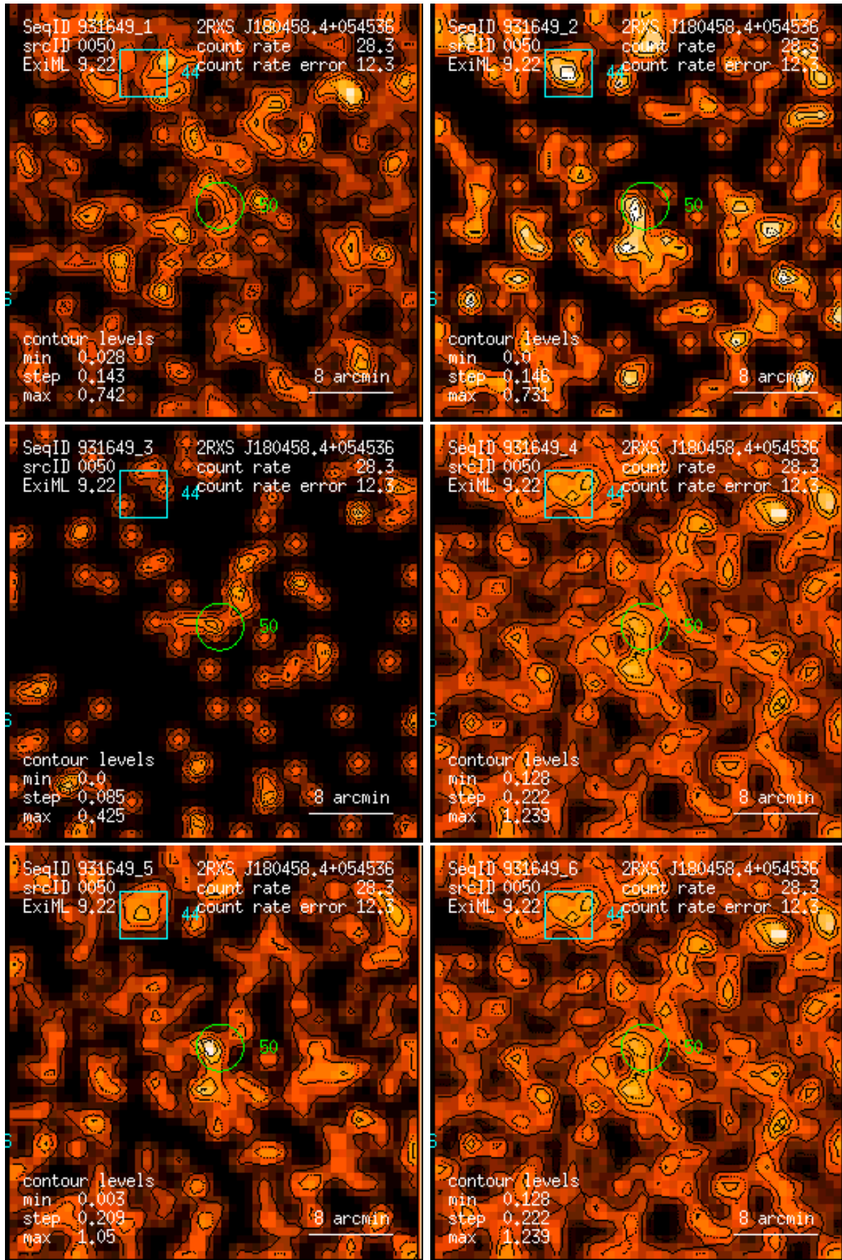
Figure 50: RASS 931649: detection 0050: band rate images, Gaussian filter: (1) PSPC channels 11 – 41, (2) 52 – 90, (3) 91 – 201, (4) 11 – 235, (5) 52 – 201, (6) 11 – 201. Broad band rates in counts/ks. Band rate contour levels in counts/ks/arcmin 2 .
