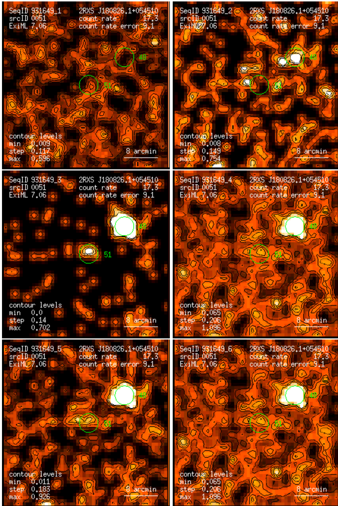
Figure 51: RASS 931649: detection 0051: band rate images, Gaussian filter: (1) PSPC channels 11 – 41, (2) 52 – 90, (3) 91 – 201, (4) 11 – 235, (5) 52 – 201, (6) 11 – 201. Broad band rates in counts/ks. Band rate contour levels in counts/ks/arcmin 2 .
