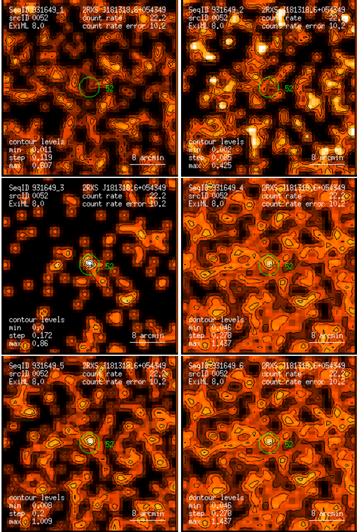
Figure 52: RASS 931649: detection 0052: band rate images, Gaussian filter: (1) PSPC channels 11 – 41, (2) 52 – 90, (3) 91 – 201, (4) 11 – 235, (5) 52 – 201, (6) 11 – 201. Broad band rates in counts/ks. Band rate contour levels in counts/ks/arcmin 2 .
