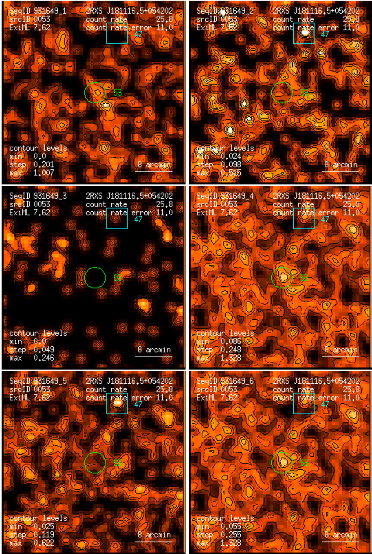
Figure 53: RASS 931649: detection 0053: band rate images, Gaussian filter: (1) PSPC channels 11 – 41, (2) 52 – 90, (3) 91 – 201, (4) 11 – 235, (5) 52 – 201, (6) 11 – 201. Broad band rates in counts/ks. Band rate contour levels in counts/ks/arcmin 2 .
