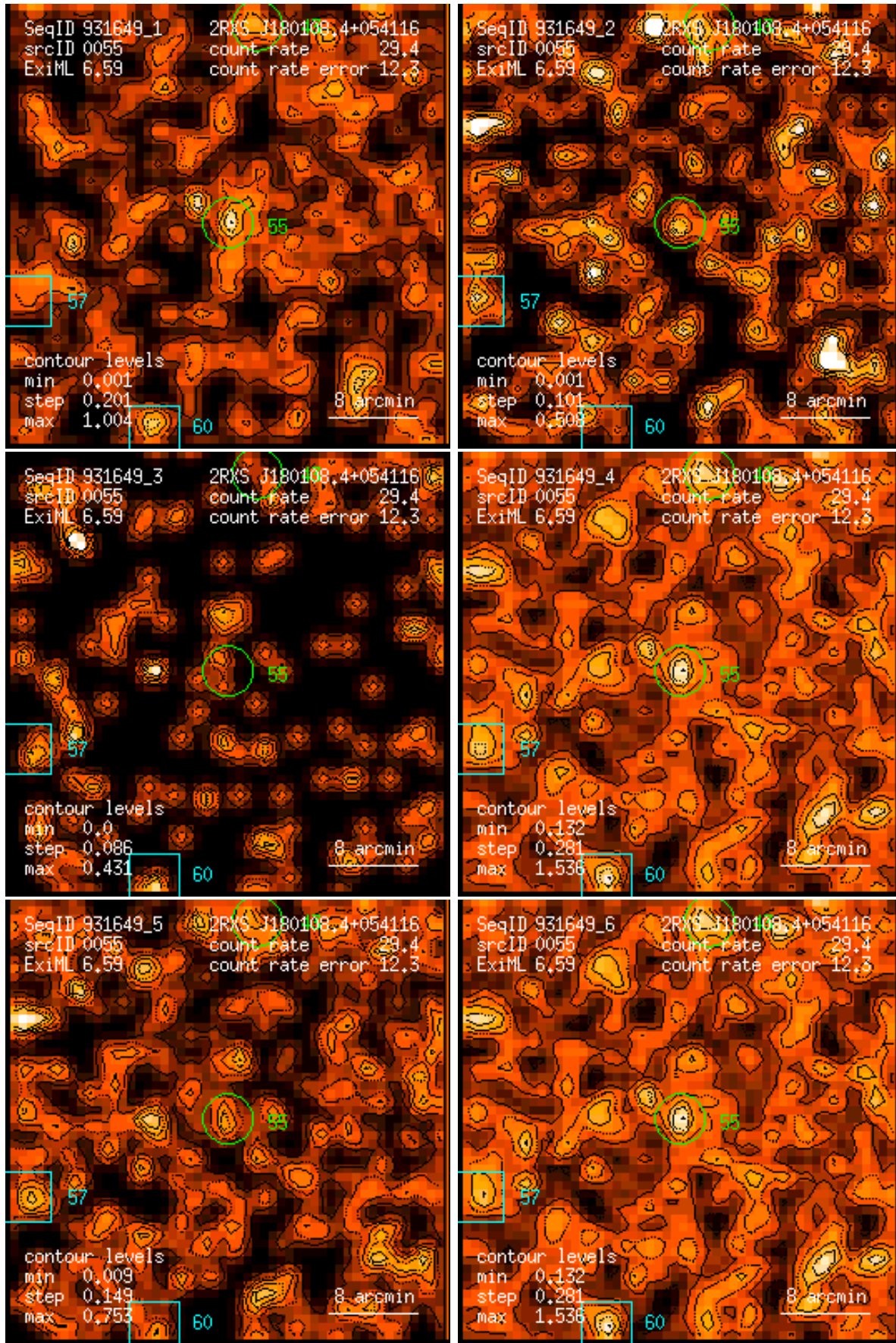
Figure 55: RASS 931649: detection 0055: band rate images, Gaussian filter: (1) PSPC channels 11 – 41, (2) 52 – 90, (3) 91 – 201, (4) 11 – 235, (5) 52 – 201, (6) 11 – 201. Broad band rates in counts/ks. Band rate contour levels in counts/ks/arcmin 2 .
