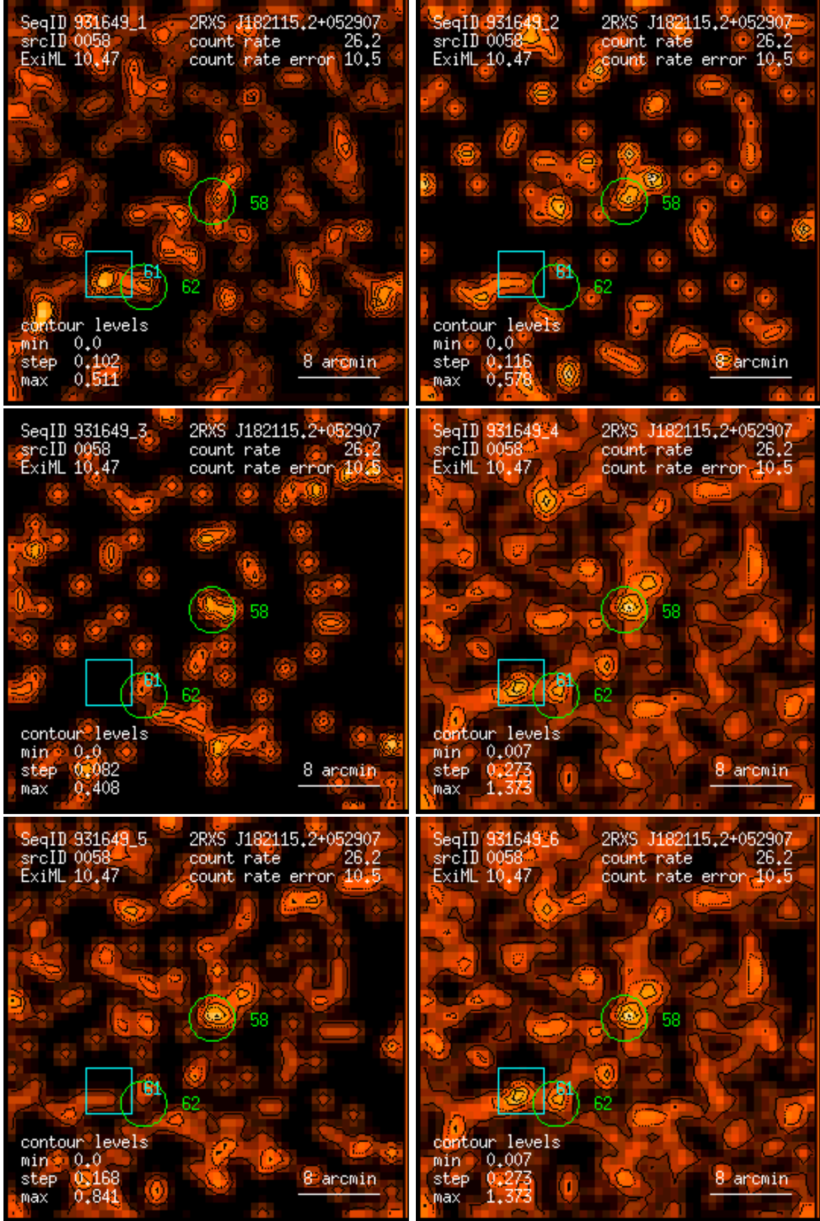
Figure 58: RASS 931649: detection 0058: band rate images, Gaussian filter: (1) PSPC channels 11 – 41, (2) 52 – 90, (3) 91 – 201, (4) 11 – 235, (5) 52 – 201, (6) 11 – 201. Broad band rates in counts/ks. Band rate contour levels in counts/ks/arcmin 2 .
