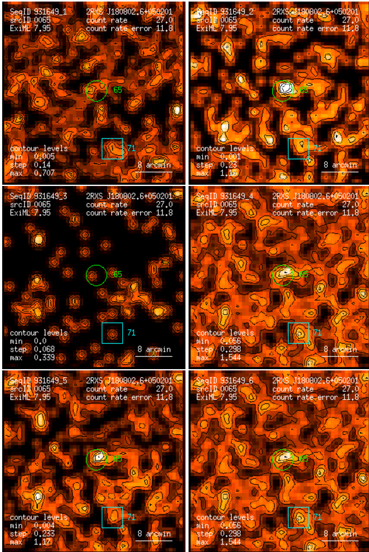
Figure 65: RASS 931649: detection 0065: band rate images, Gaussian filter: (1) PSPC channels 11 – 41, (2) 52 – 90, (3) 91 – 201, (4) 11 – 235, (5) 52 – 201, (6) 11 – 201. Broad band rates in counts/ks. Band rate contour levels in counts/ks/arcmin 2 .
