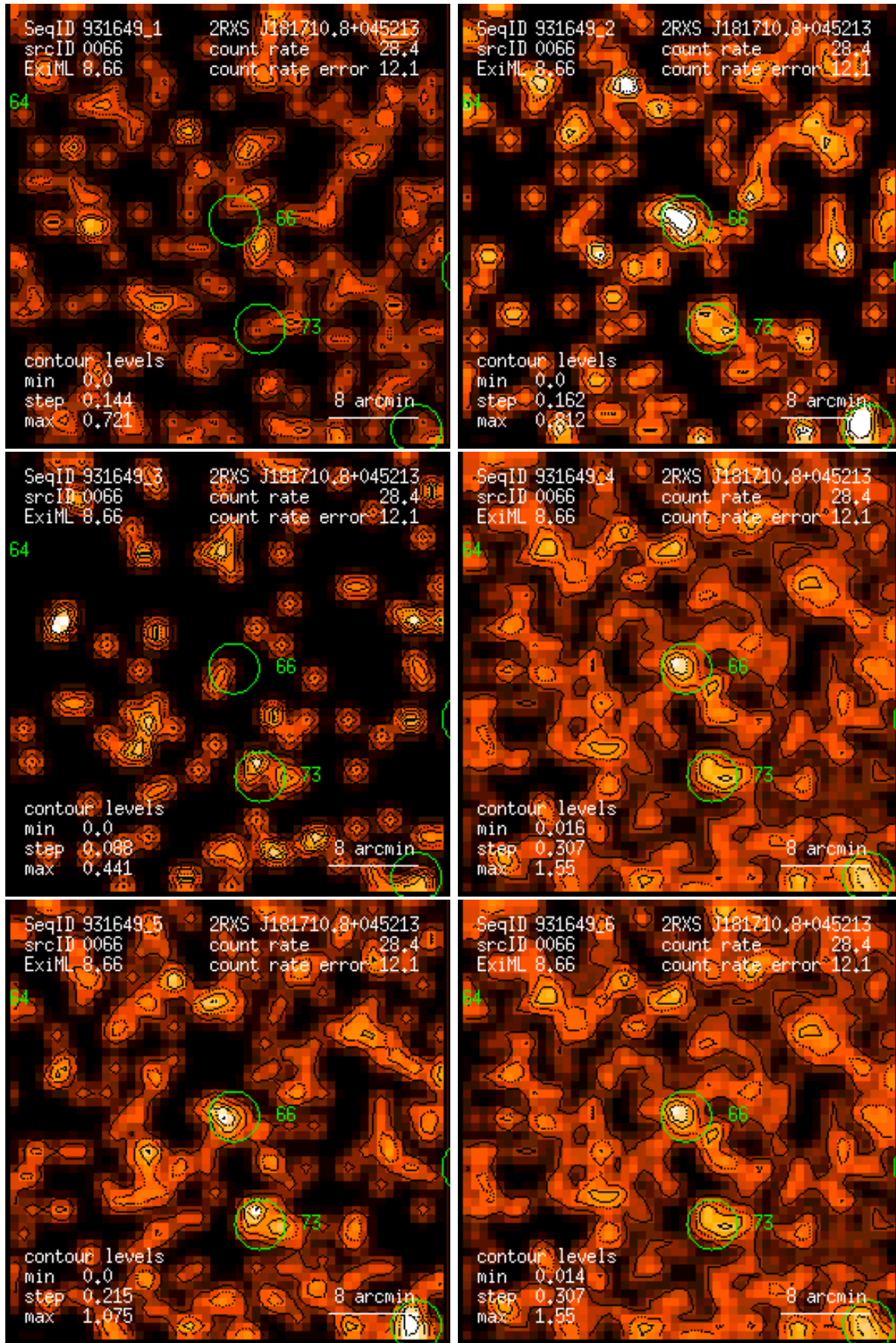
Figure 66: RASS 931649: detection 0066: band rate images, Gaussian filter: (1) PSPC channels 11 – 41, (2) 52 – 90, (3) 91 – 201, (4) 11 – 235, (5) 52 – 201, (6) 11 – 201. Broad band rates in counts/ks. Band rate contour levels in counts/ks/arcmin 2 .
