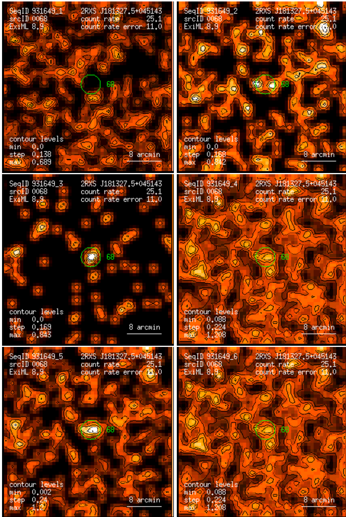
Figure 68: RASS 931649: detection 0068: band rate images, Gaussian filter: (1) PSPC channels 11 – 41, (2) 52 – 90, (3) 91 – 201, (4) 11 – 235, (5) 52 – 201, (6) 11 – 201. Broad band rates in counts/ks. Band rate contour levels in counts/ks/arcmin 2 .
