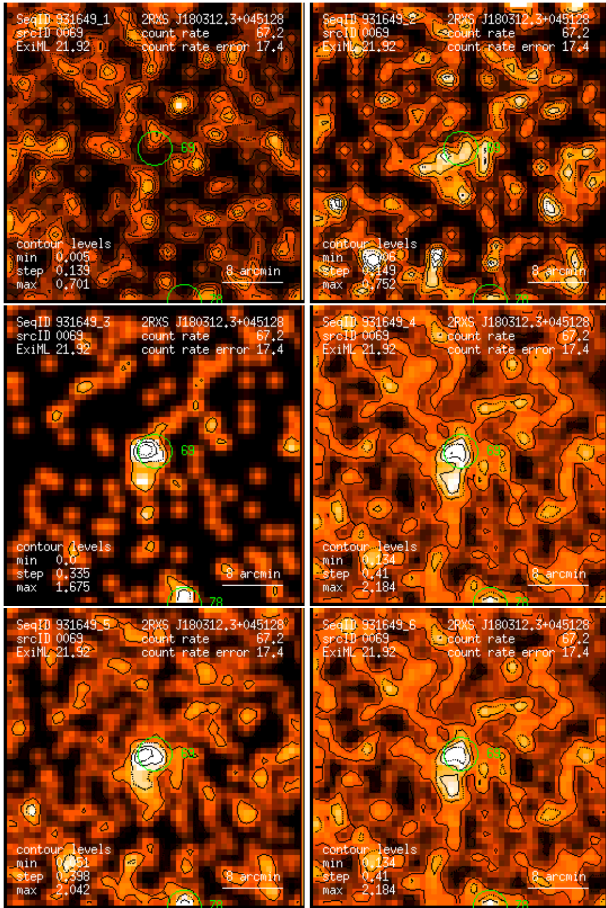
Figure 69: RASS 931649: detection 0069: band rate images, Gaussian filter: (1) PSPC channels 11 – 41, (2) 52 – 90, (3) 91 – 201, (4) 11 – 235, (5) 52 – 201, (6) 11 – 201. Broad band rates in counts/ks. Band rate contour levels in counts/ks/arcmin 2 .
