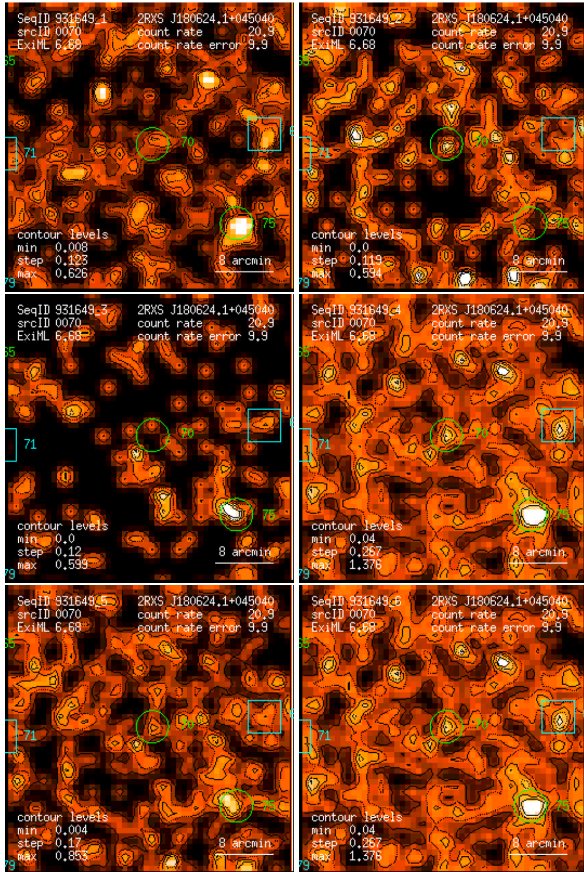
Figure 70: RASS 931649: detection 0070: band rate images, Gaussian filter: (1) PSPC channels 11 – 41, (2) 52 – 90, (3) 91 – 201, (4) 11 – 235, (5) 52 – 201, (6) 11 – 201. Broad band rates in counts/ks. Band rate contour levels in counts/ks/arcmin 2 .
