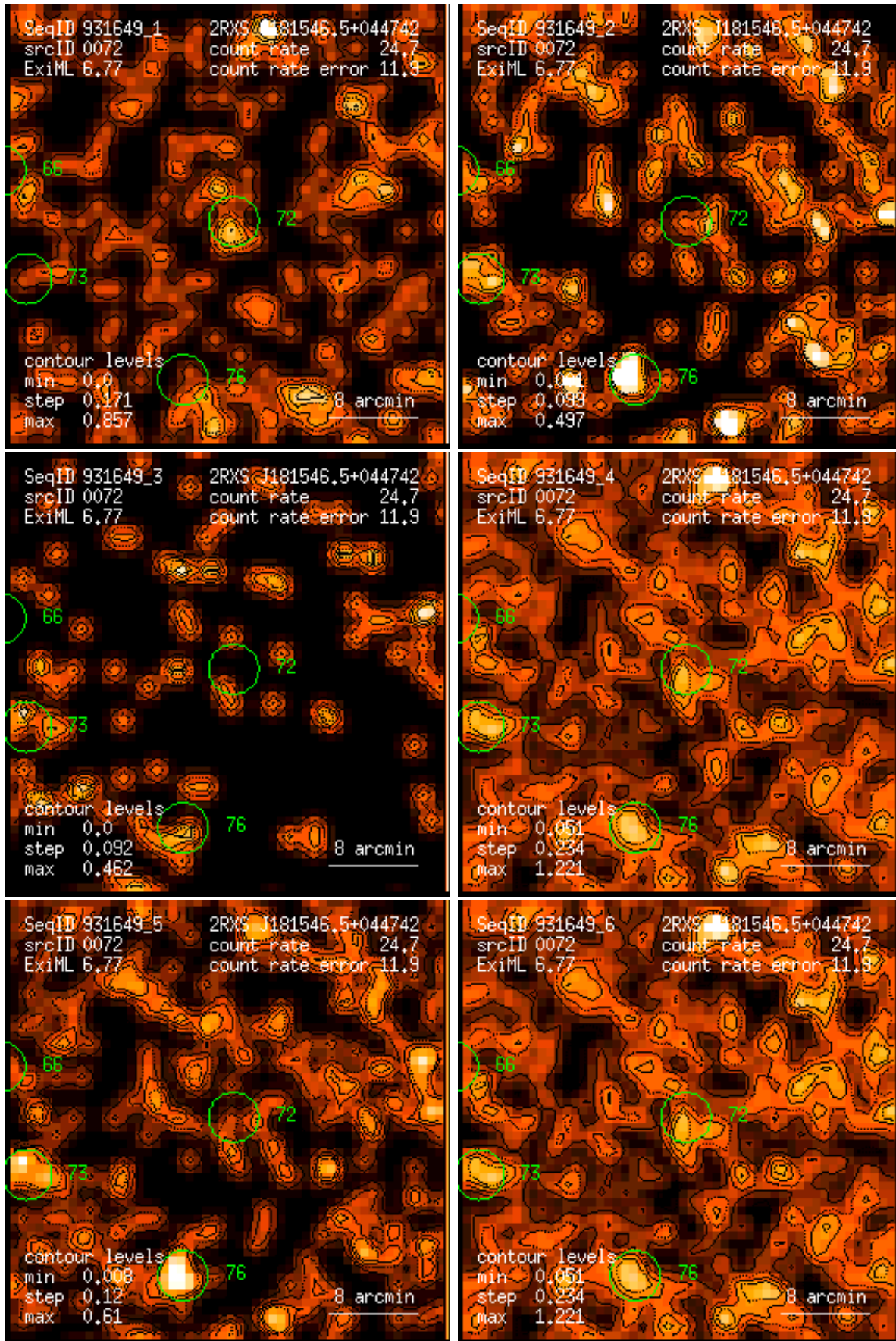
Figure 72: RASS 931649: detection 0072: band rate images, Gaussian filter: (1) PSPC channels 11 – 41, (2) 52 – 90, (3) 91 – 201, (4) 11 – 235, (5) 52 – 201, (6) 11 – 201. Broad band rates in counts/ks. Band rate contour levels in counts/ks/arcmin 2 .
