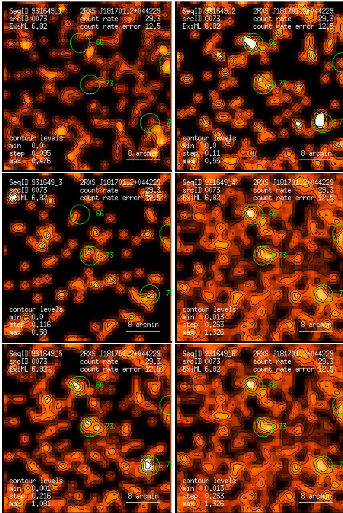
Figure 73: RASS 931649: detection 0073: band rate images, Gaussian filter: (1) PSPC channels 11 – 41, (2) 52 – 90, (3) 91 – 201, (4) 11 – 235, (5) 52 – 201, (6) 11 – 201. Broad band rates in counts/ks. Band rate contour levels in counts/ks/arcmin 2 .
