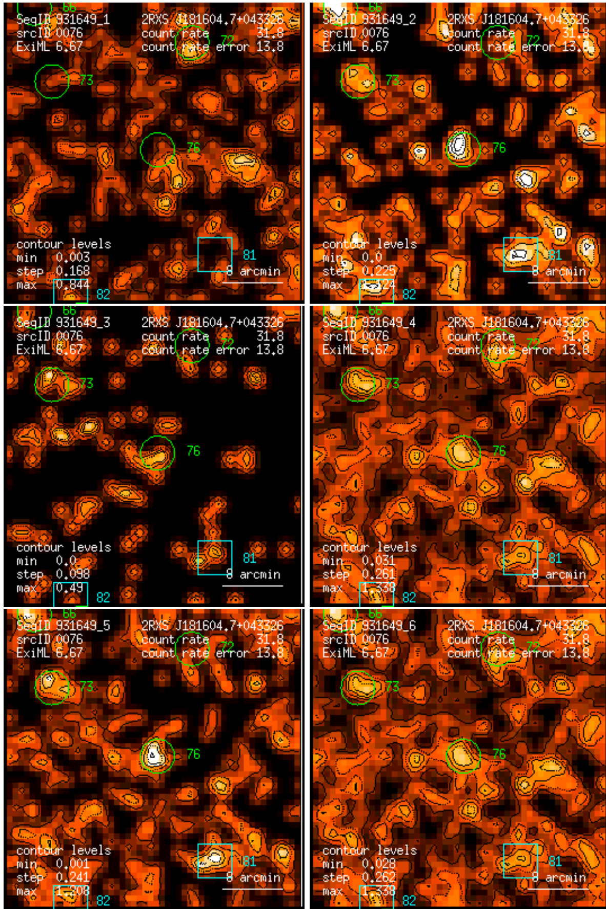
Figure 76: RASS 931649: detection 0076: band rate images, Gaussian filter: (1) PSPC channels 11 – 41, (2) 52 – 90, (3) 91 – 201, (4) 11 – 235, (5) 52 – 201, (6) 11 – 201. Broad band rates in counts/ks. Band rate contour levels in counts/ks/arcmin 2 .
