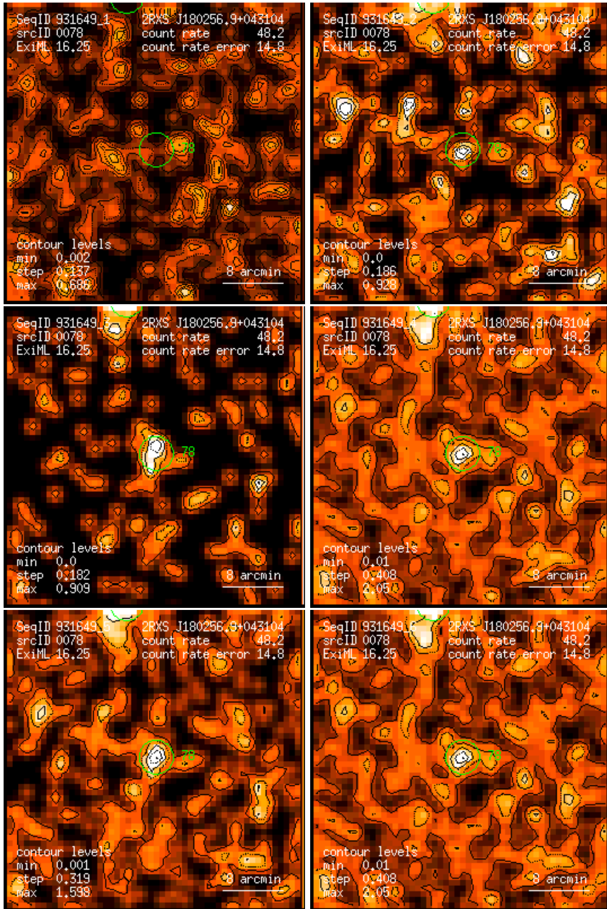
Figure 78: RASS 931649: detection 0078: band rate images, Gaussian filter: (1) PSPC channels 11 – 41, (2) 52 – 90, (3) 91 – 201, (4) 11 – 235, (5) 52 – 201, (6) 11 – 201. Broad band rates in counts/ks. Band rate contour levels in counts/ks/arcmin 2 .
