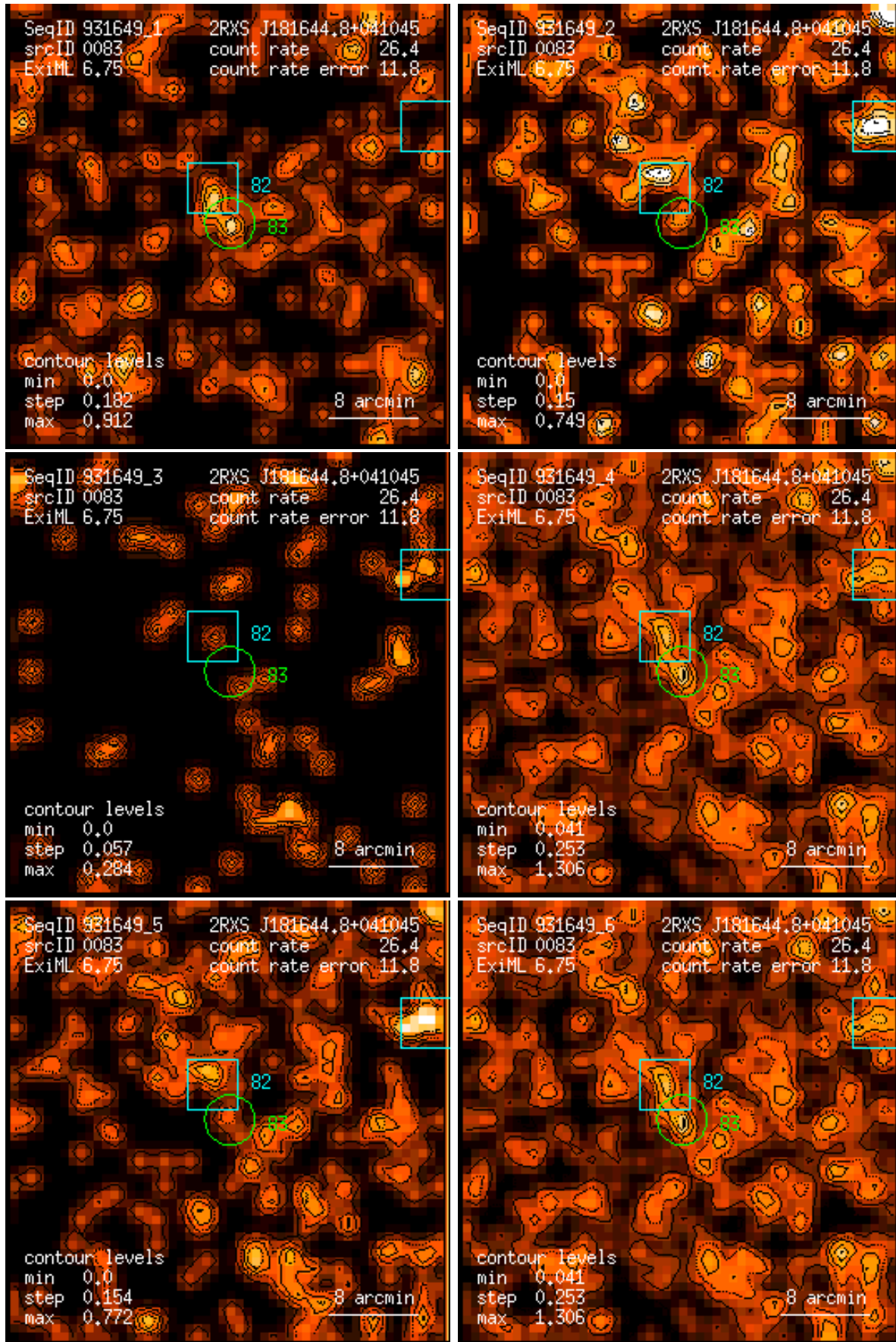
Figure 83: RASS 931649: detection 0083: band rate images, Gaussian filter: (1) PSPC channels 11 – 41, (2) 52 – 90, (3) 91 – 201, (4) 11 – 235, (5) 52 – 201, (6) 11 – 201. Broad band rates in counts/ks. Band rate contour levels in counts/ks/arcmin 2 .
