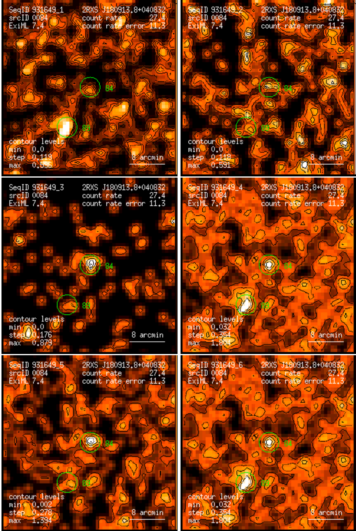
Figure 84: RASS 931649: detection 0084: band rate images, Gaussian filter: (1) PSPC channels 11 – 41, (2) 52 – 90, (3) 91 – 201, (4) 11 – 235, (5) 52 – 201, (6) 11 – 201. Broad band rates in counts/ks. Band rate contour levels in counts/ks/arcmin 2 .
