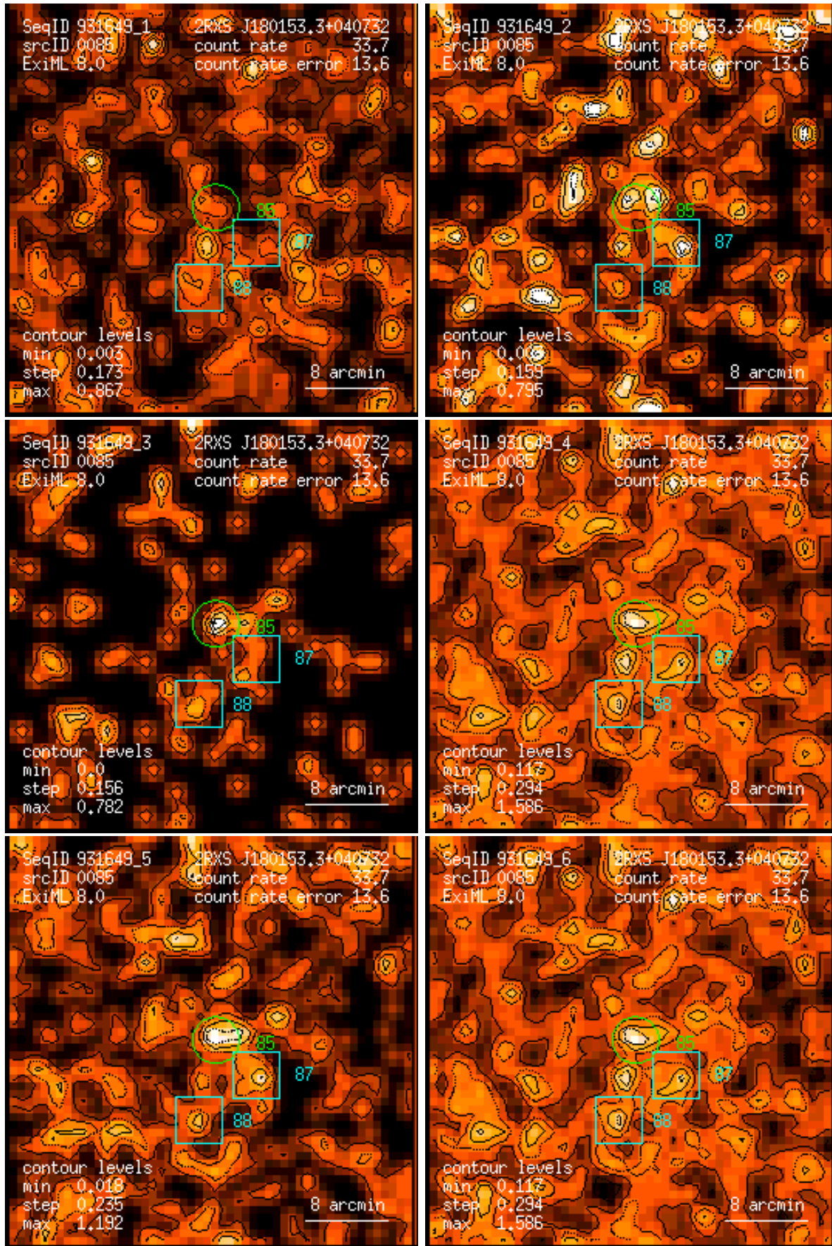
Figure 85: RASS 931649: detection 0085: band rate images, Gaussian filter: (1) PSPC channels 11 – 41, (2) 52 – 90, (3) 91 – 201, (4) 11 – 235, (5) 52 – 201, (6) 11 – 201. Broad band rates in counts/ks. Band rate contour levels in counts/ks/arcmin 2 .
