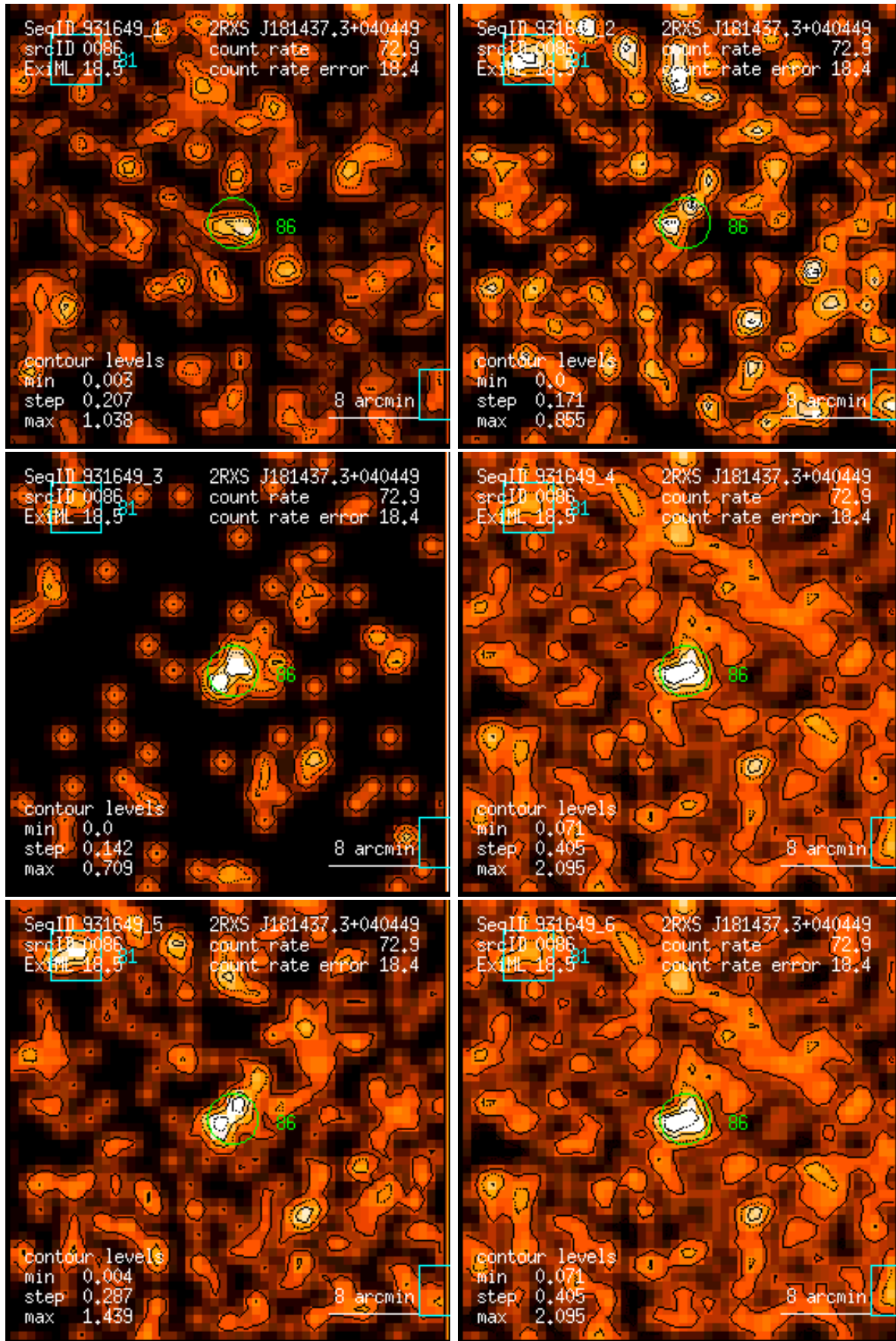
Figure 86: RASS 931649: detection 0086: band rate images, Gaussian filter: (1) PSPC channels 11 – 41, (2) 52 – 90, (3) 91 – 201, (4) 11 – 235, (5) 52 – 201, (6) 11 – 201. Broad band rates in counts/ks. Band rate contour levels in counts/ks/arcmin 2 .
