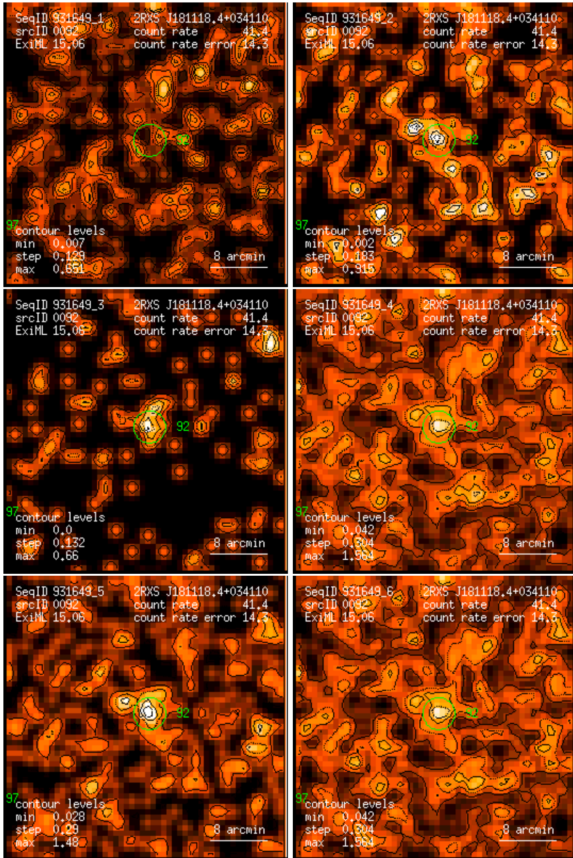
Figure 92: RASS 931649: detection 0092: band rate images, Gaussian filter: (1) PSPC channels 11 – 41, (2) 52 – 90, (3) 91 – 201, (4) 11 – 235, (5) 52 – 201, (6) 11 – 201. Broad band rates in counts/ks. Band rate contour levels in counts/ks/arcmin 2 .
