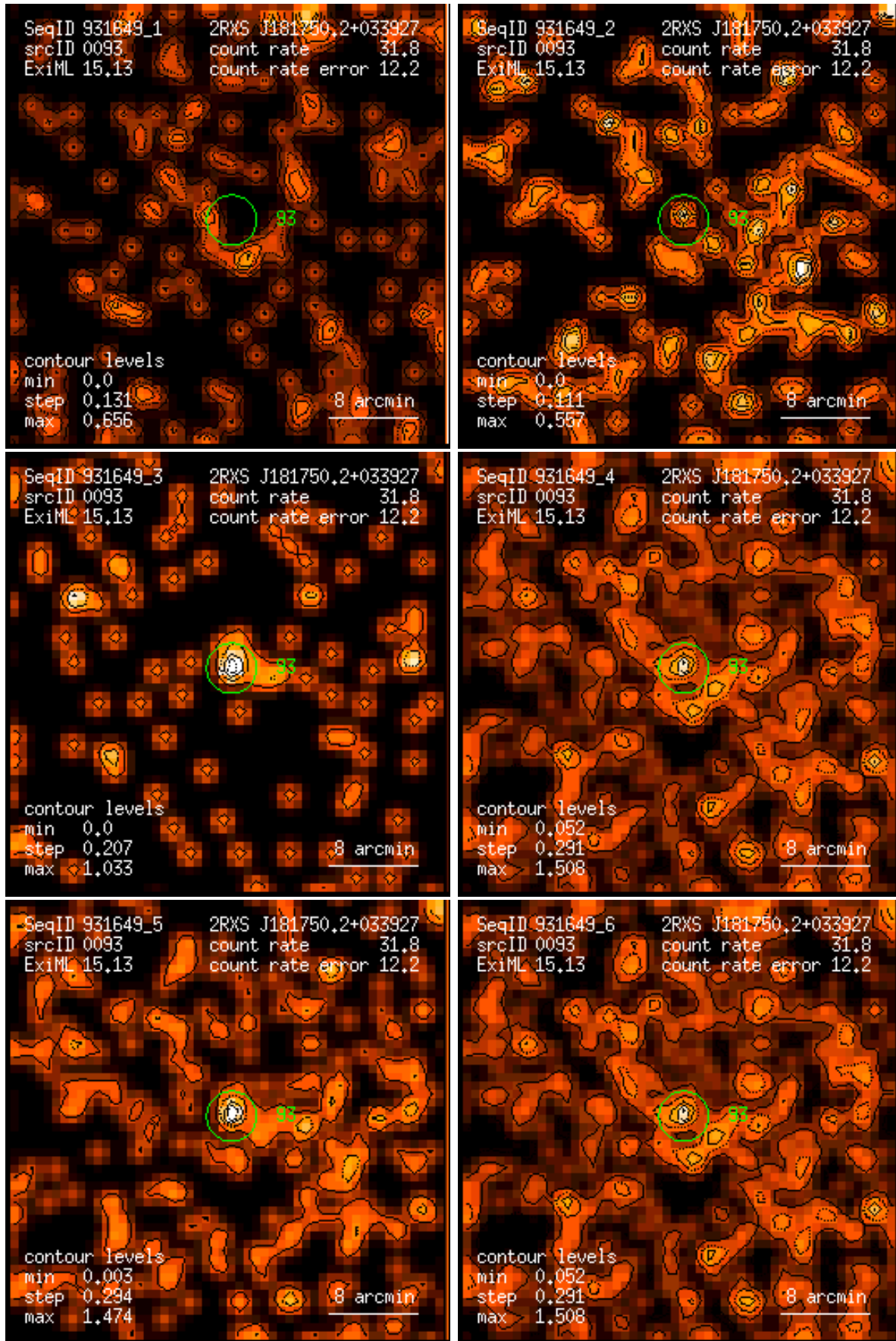
Figure 93: RASS 931649: detection 0093: band rate images, Gaussian filter: (1) PSPC channels 11 – 41, (2) 52 – 90, (3) 91 – 201, (4) 11 – 235, (5) 52 – 201, (6) 11 – 201. Broad band rates in counts/ks. Band rate contour levels in counts/ks/arcmin 2 .
