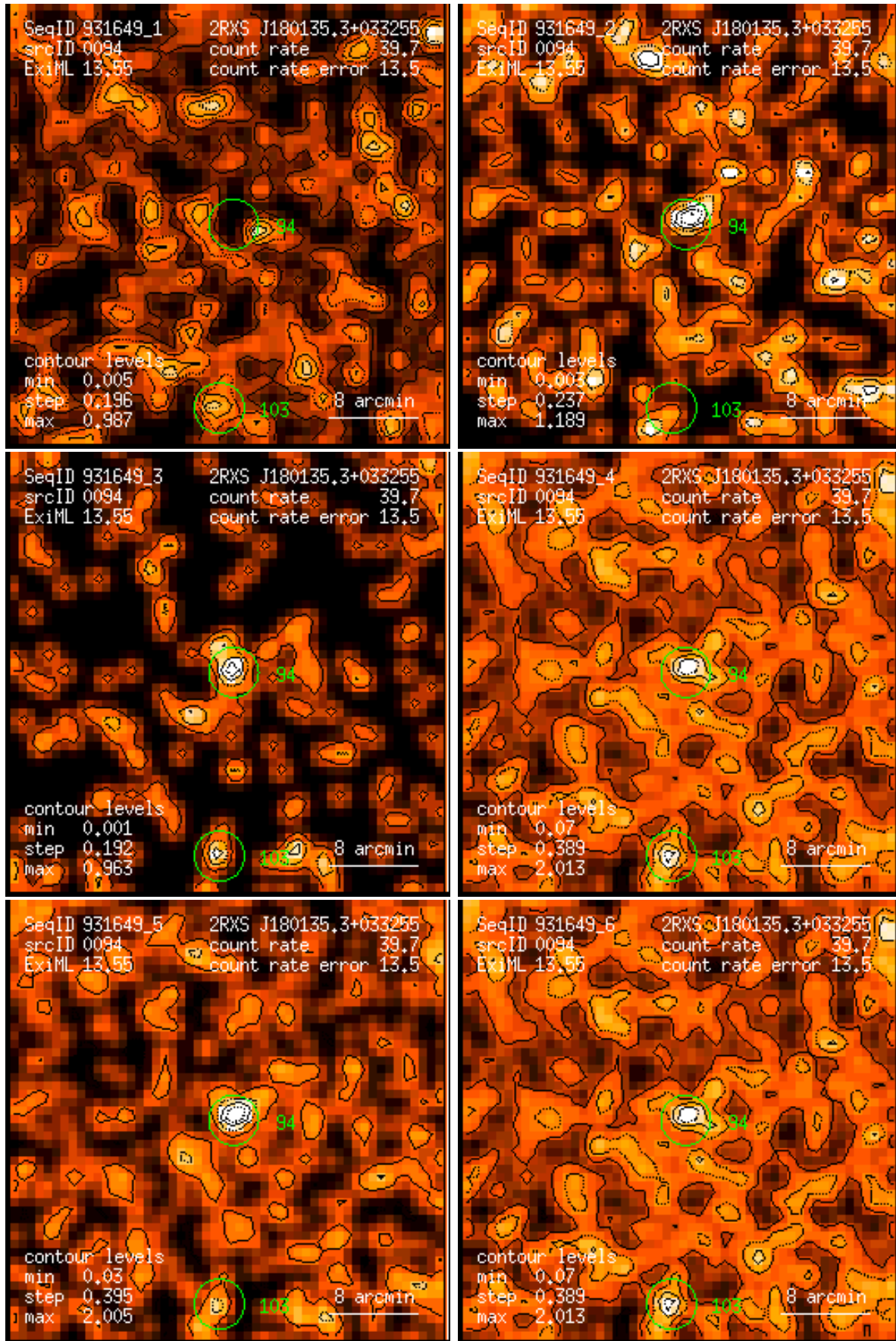
Figure 94: RASS 931649: detection 0094: band rate images, Gaussian filter: (1) PSPC channels 11 – 41, (2) 52 – 90, (3) 91 – 201, (4) 11 – 235, (5) 52 – 201, (6) 11 – 201. Broad band rates in counts/ks. Band rate contour levels in counts/ks/arcmin 2 .
