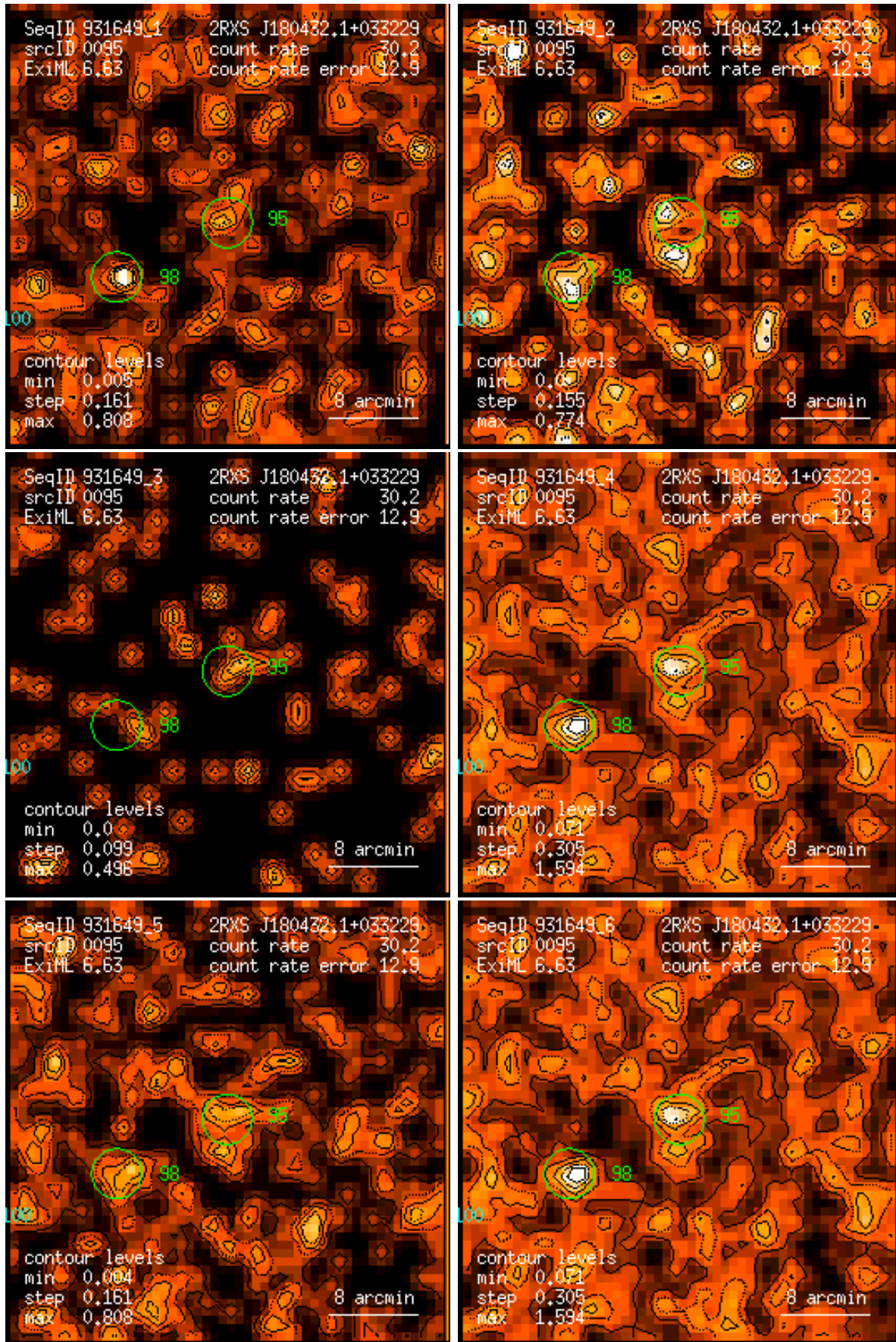
Figure 95: RASS 931649: detection 0095: band rate images, Gaussian filter: (1) PSPC channels 11 – 41, (2) 52 – 90, (3) 91 – 201, (4) 11 – 235, (5) 52 – 201, (6) 11 – 201. Broad band rates in counts/ks. Band rate contour levels in counts/ks/arcmin 2 .
