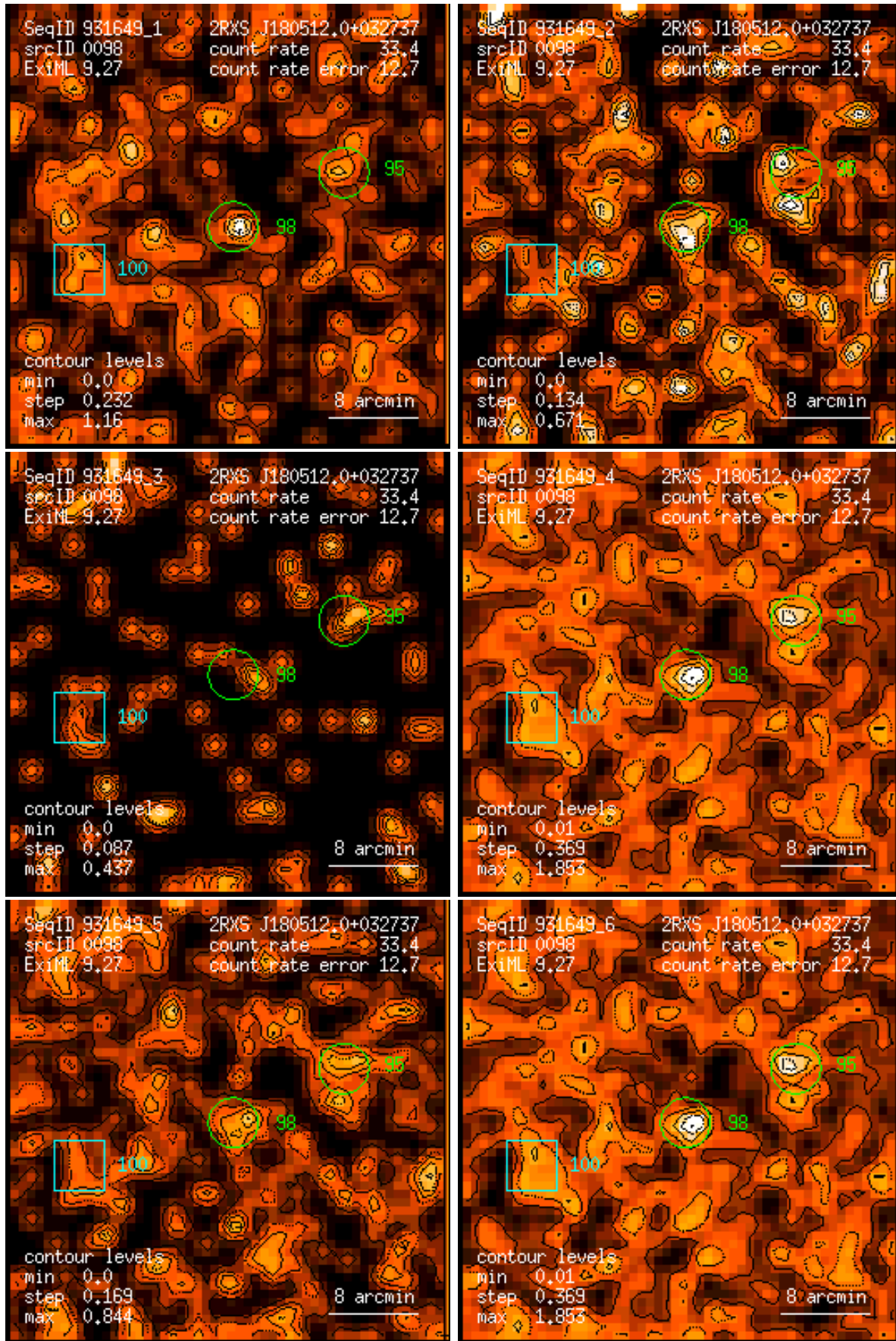
Figure 98: RASS 931649: detection 0098: band rate images, Gaussian filter: (1) PSPC channels 11 – 41, (2) 52 – 90, (3) 91 – 201, (4) 11 – 235, (5) 52 – 201, (6) 11 – 201. Broad band rates in counts/ks. Band rate contour levels in counts/ks/arcmin 2 .
