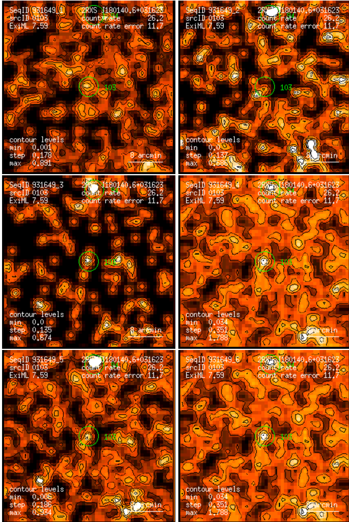
Figure 103: RASS 931649: detection 0103: band rate images, Gaussian filter: (1) PSPC channels 11 – 41, (2) 52 – 90, (3) 91 – 201, (4) 11 – 235, (5) 52 – 201, (6) 11 – 201. Broad band rates in counts/ks. Band rate contour levels in counts/ks/arcmin 2 .
