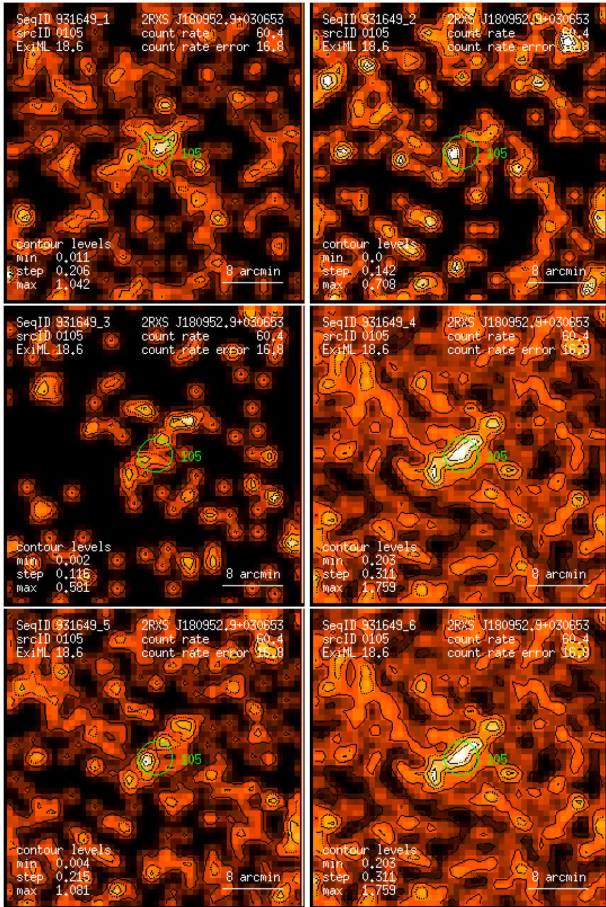
Figure 105: RASS 931649: detection 0105: band rate images, Gaussian filter: (1) PSPC channels 11 – 41, (2) 52 – 90, (3) 91 – 201, (4) 11 – 235, (5) 52 – 201, (6) 11 – 201. Broad band rates in counts/ks. Band rate contour levels in counts/ks/arcmin 2 .
