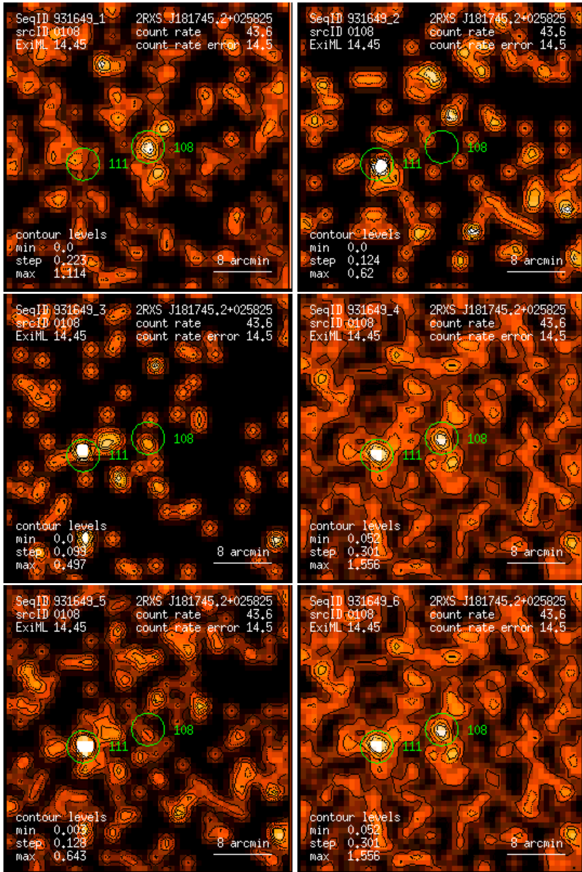
Figure 108: RASS 931649: detection 0108: band rate images, Gaussian filter: (1) PSPC channels 11 – 41, (2) 52 – 90, (3) 91 – 201, (4) 11 – 235, (5) 52 – 201, (6) 11 – 201. Broad band rates in counts/ks. Band rate contour levels in counts/ks/arcmin 2 .
