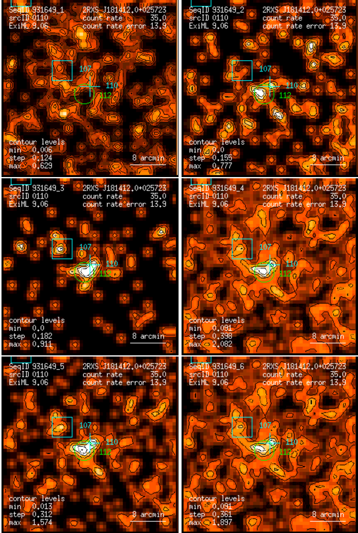
Figure 110: RASS 931649: detection 0110: band rate images, Gaussian filter: (1) PSPC channels 11 – 41, (2) 52 – 90, (3) 91 – 201, (4) 11 – 235, (5) 52 – 201, (6) 11 – 201. Broad band rates in counts/ks. Band rate contour levels in counts/ks/arcmin 2 .
