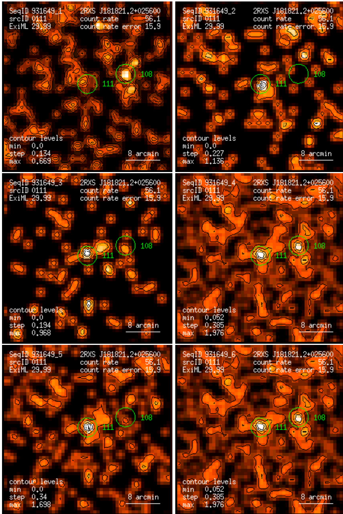
Figure 111: RASS 931649: detection 0111: band rate images, Gaussian filter: (1) PSPC channels 11 – 41, (2) 52 – 90, (3) 91 – 201, (4) 11 – 235, (5) 52 – 201, (6) 11 – 201. Broad band rates in counts/ks. Band rate contour levels in counts/ks/arcmin 2 .
