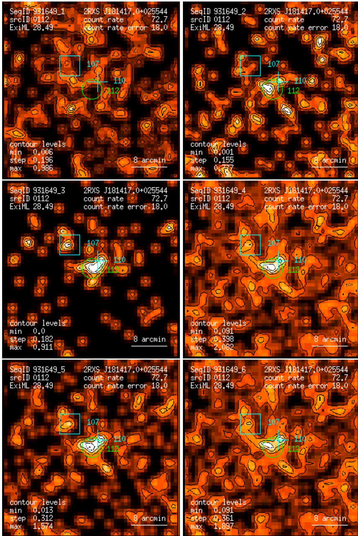
Figure 112: RASS 931649: detection 0112: band rate images, Gaussian filter: (1) PSPC channels 11 – 41, (2) 52 – 90, (3) 91 – 201, (4) 11 – 235, (5) 52 – 201, (6) 11 – 201. Broad band rates in counts/ks. Band rate contour levels in counts/ks/arcmin 2 .
