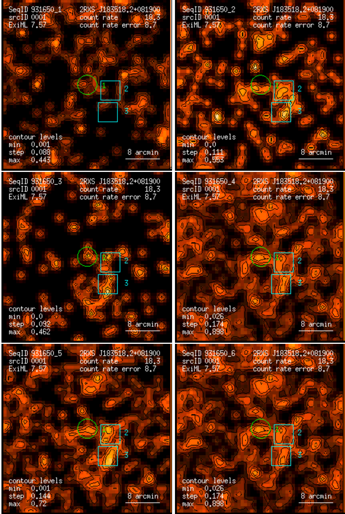
Figure 1: RASS 931650: detection 0001: band rate images, Gaussian filter: (1) PSPC channels 11 – 41, (2) 52 – 90, (3) 91 – 201, (4) 11 – 235, (5) 52 – 201, (6) 11 – 201. Broad band rates in counts/ks. Band rate contour levels in counts/ks/arcmin 2 .
