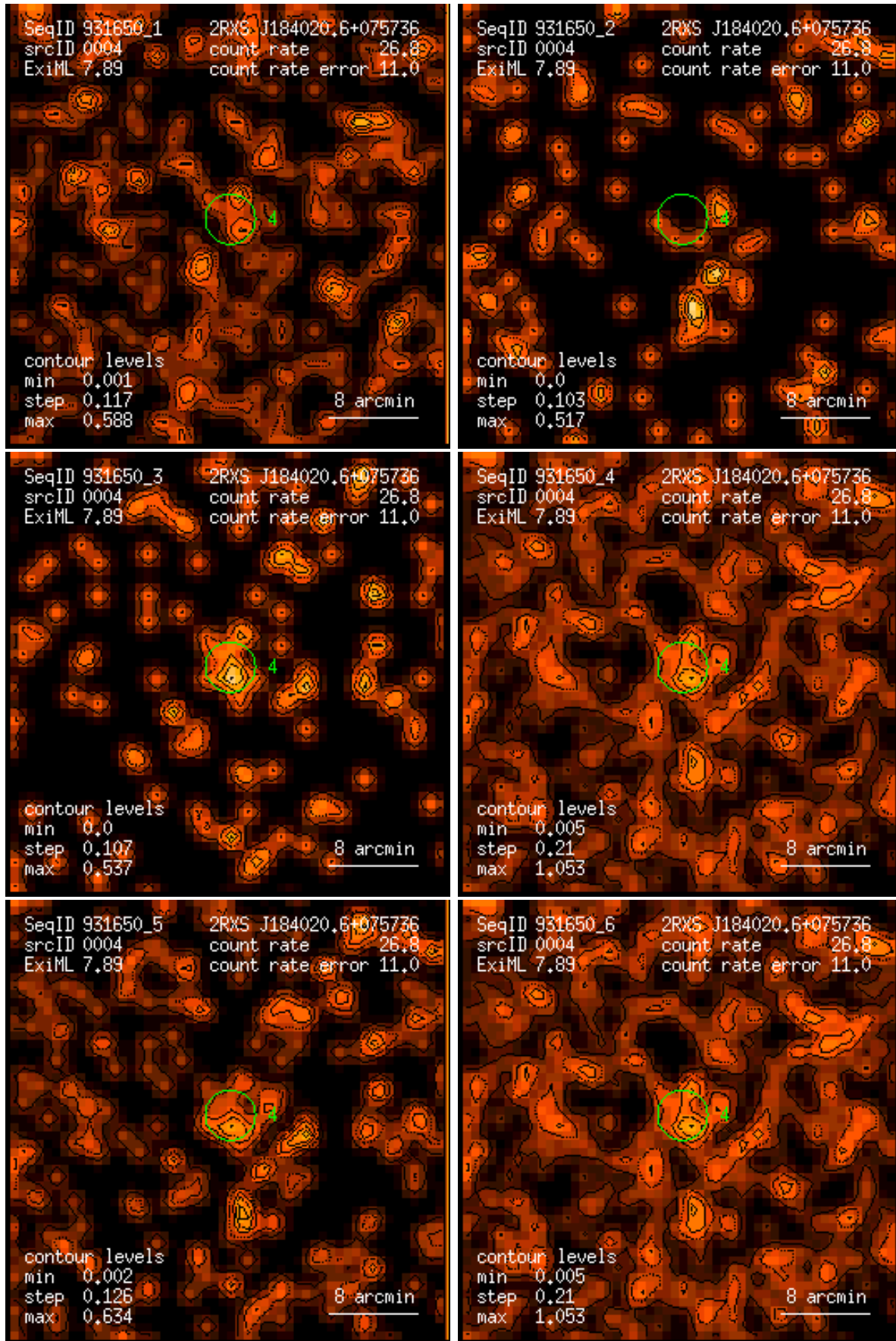
Figure 4: RASS 931650: detection 0004: band rate images, Gaussian filter: (1) PSPC channels 11 – 41, (2) 52 – 90, (3) 91 – 201, (4) 11 – 235, (5) 52 – 201, (6) 11 – 201. Broad band rates in counts/ks. Band rate contour levels in counts/ks/arcmin 2 .
