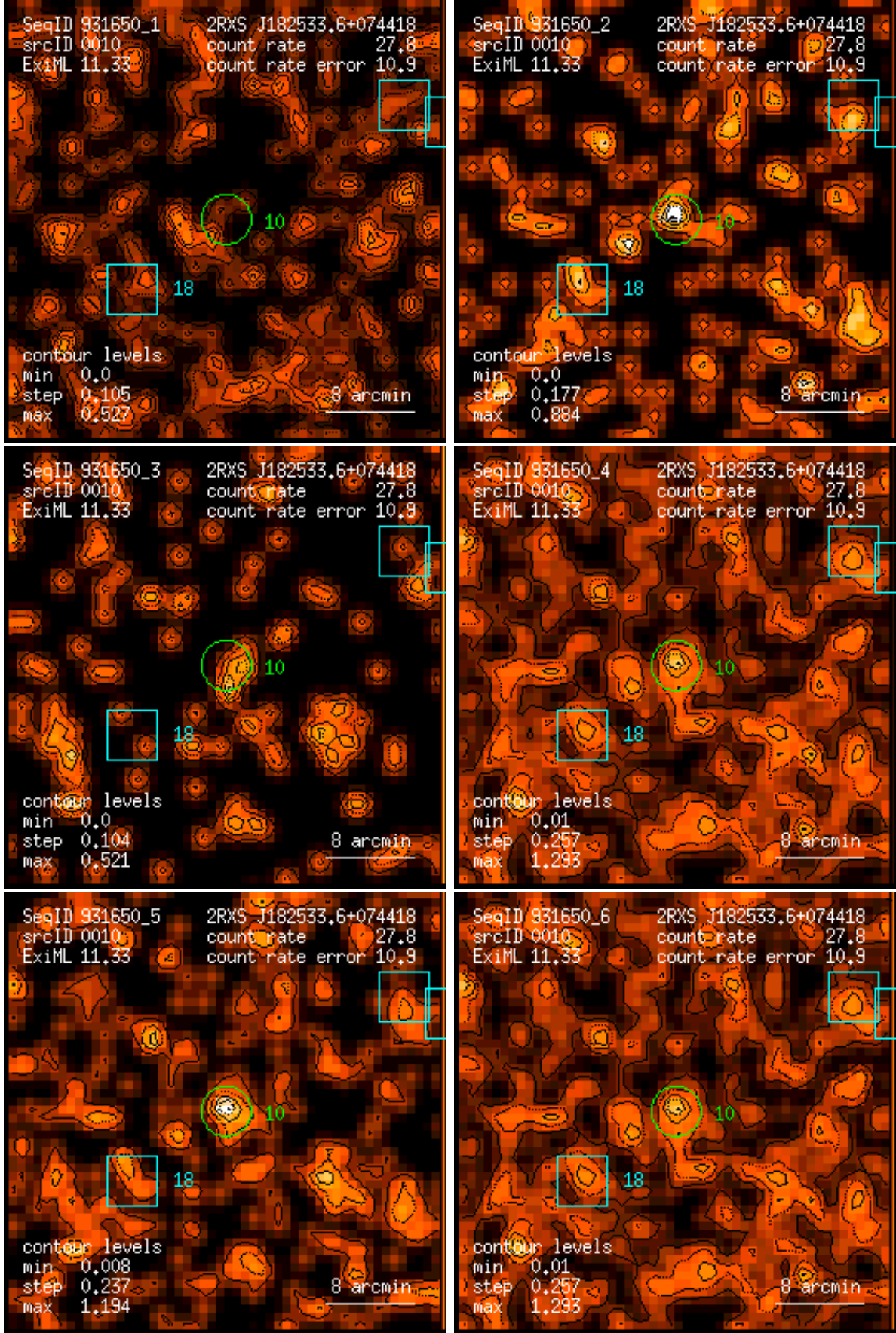
Figure 10: RASS 931650: detection 0010: band rate images, Gaussian filter: (1) PSPC channels 11 – 41, (2) 52 – 90, (3) 91 – 201, (4) 11 – 235, (5) 52 – 201, (6) 11 – 201. Broad band rates in counts/ks. Band rate contour levels in counts/ks/arcmin 2 .
