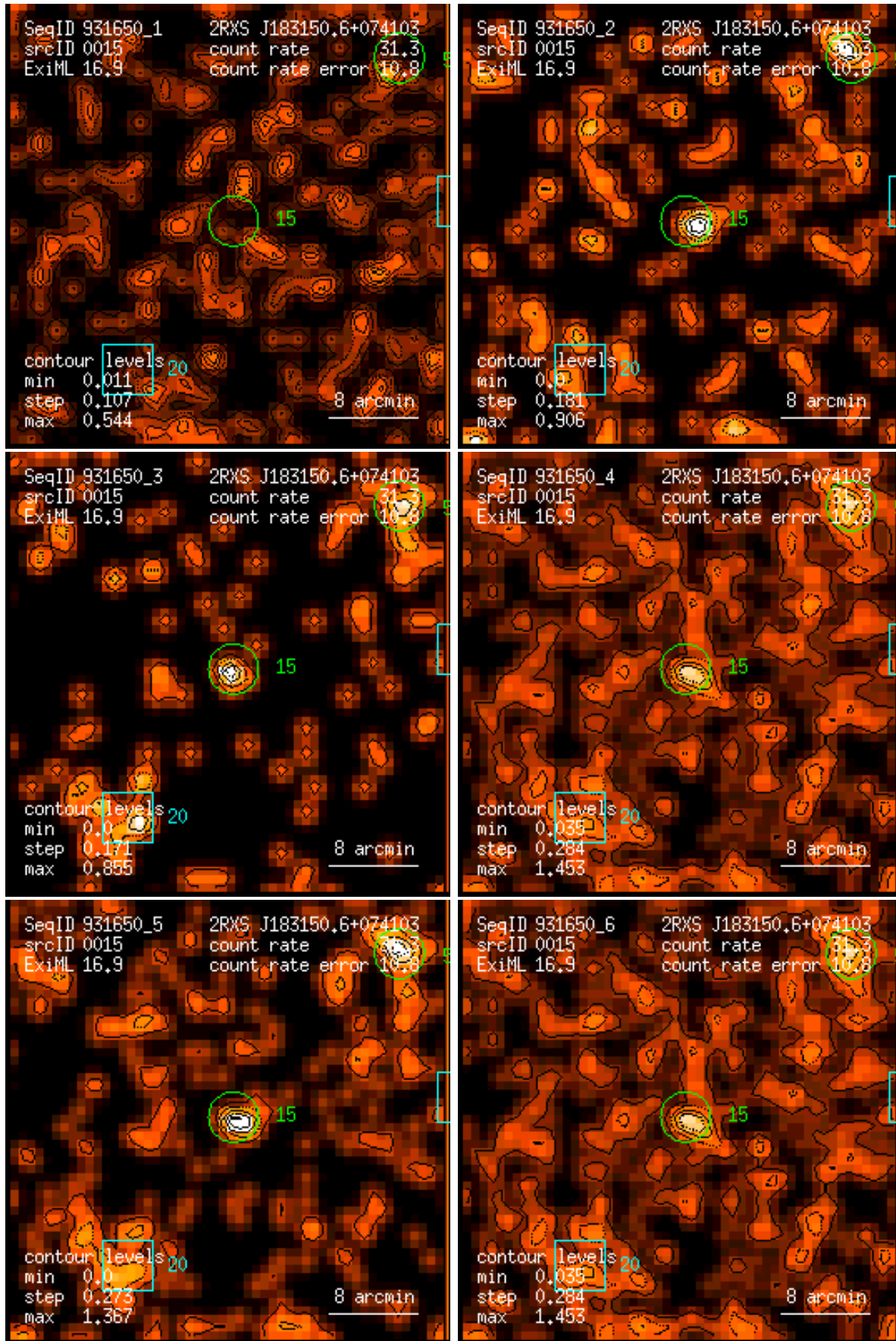
Figure 15: RASS 931650: detection 0015: band rate images, Gaussian filter: (1) PSPC channels 11 – 41, (2) 52 – 90, (3) 91 – 201, (4) 11 – 235, (5) 52 – 201, (6) 11 – 201. Broad band rates in counts/ks. Band rate contour levels in counts/ks/arcmin 2 .
