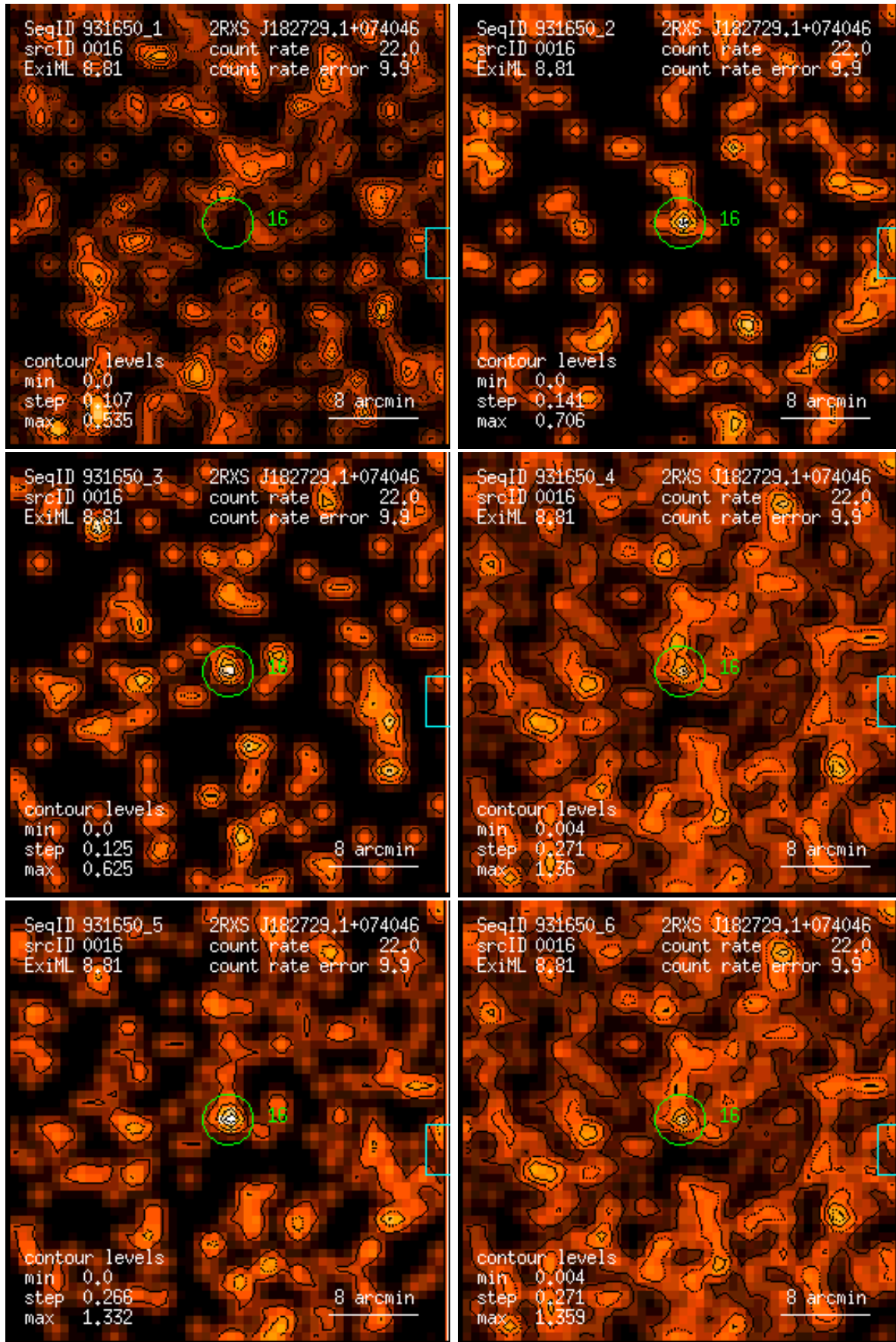
Figure 16: RASS 931650: detection 0016: band rate images, Gaussian filter: (1) PSPC channels 11 – 41, (2) 52 – 90, (3) 91 – 201, (4) 11 – 235, (5) 52 – 201, (6) 11 – 201. Broad band rates in counts/ks. Band rate contour levels in counts/ks/arcmin 2 .
