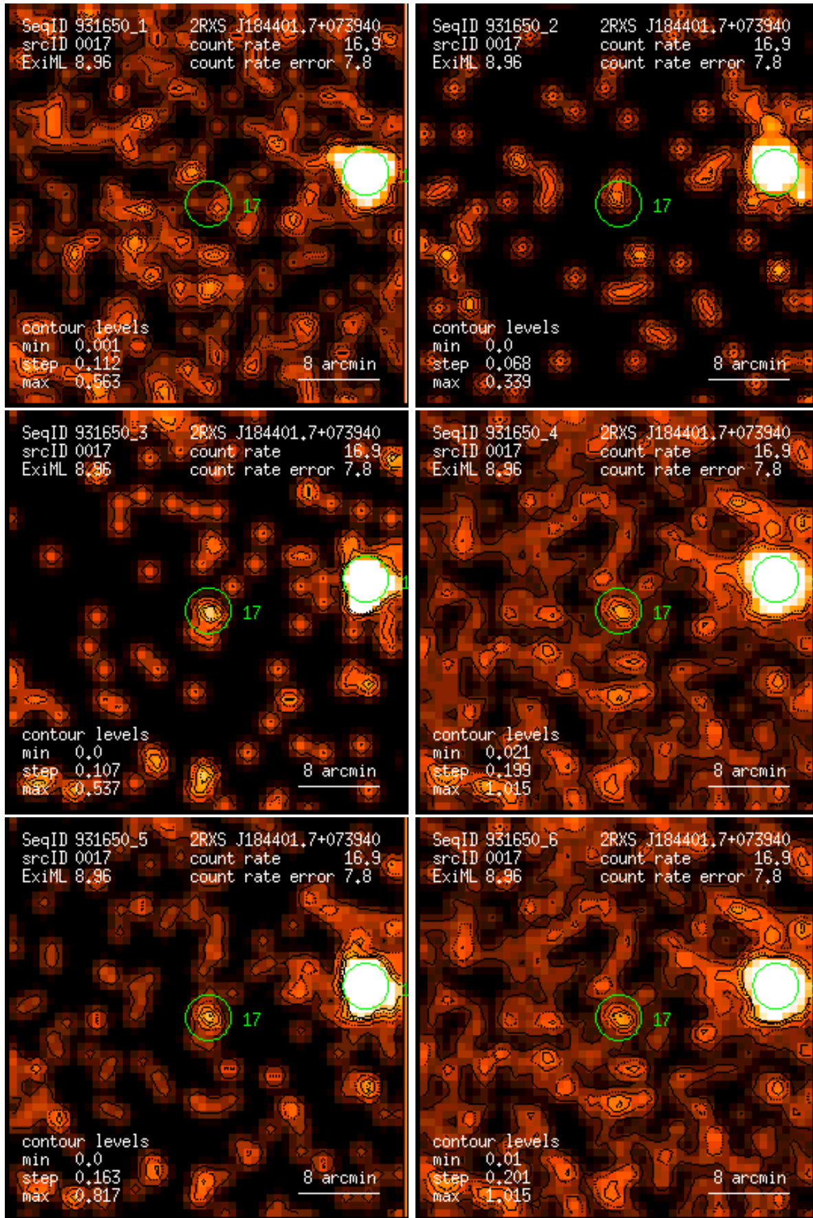
Figure 17: RASS 931650: detection 0017: band rate images, Gaussian filter: (1) PSPC channels 11 – 41, (2) 52 – 90, (3) 91 – 201, (4) 11 – 235, (5) 52 – 201, (6) 11 – 201. Broad band rates in counts/ks. Band rate contour levels in counts/ks/arcmin 2 .
