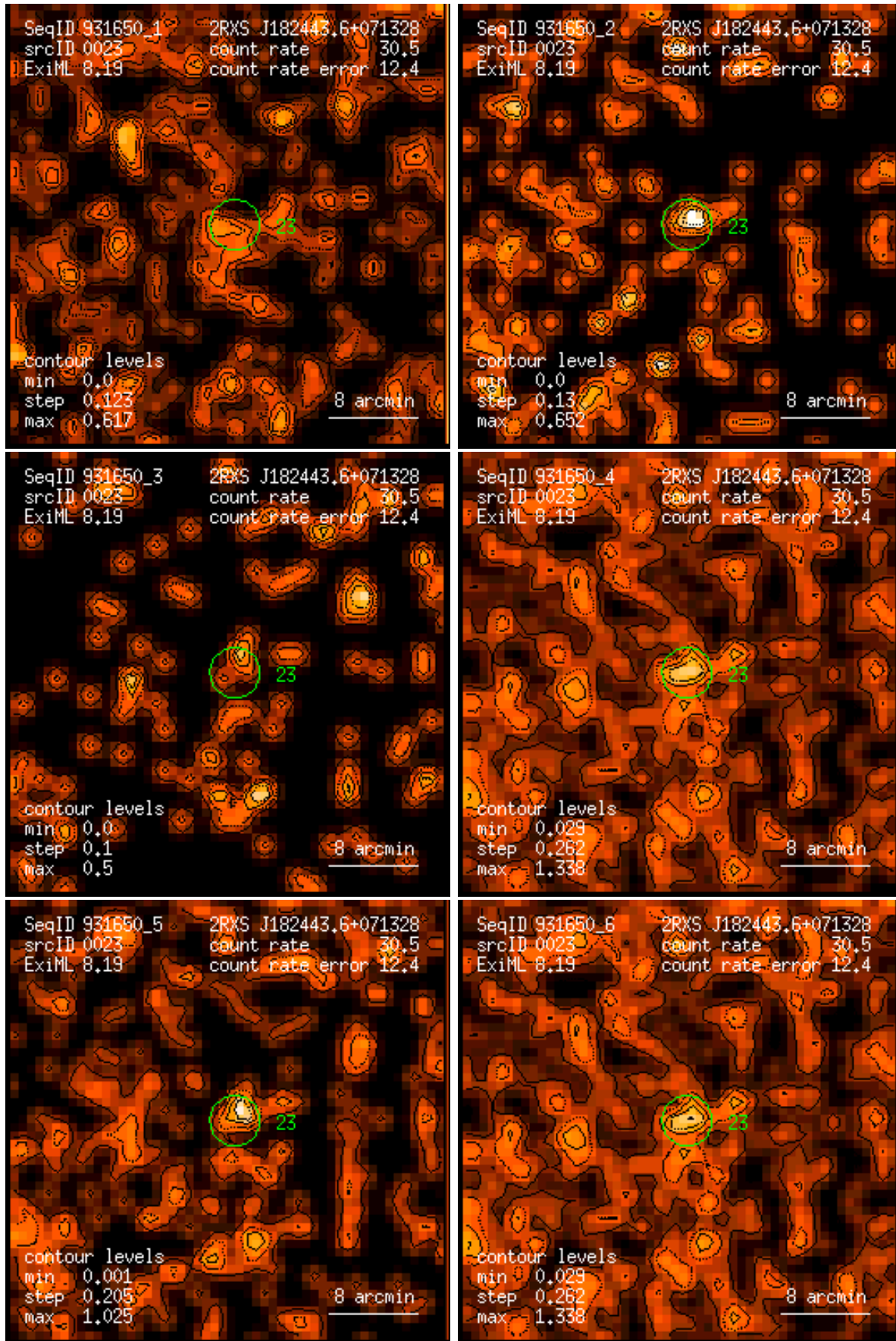
Figure 23: RASS 931650: detection 0023: band rate images, Gaussian filter: (1) PSPC channels 11 – 41, (2) 52 – 90, (3) 91 – 201, (4) 11 – 235, (5) 52 – 201, (6) 11 – 201. Broad band rates in counts/ks. Band rate contour levels in counts/ks/arcmin 2 .
