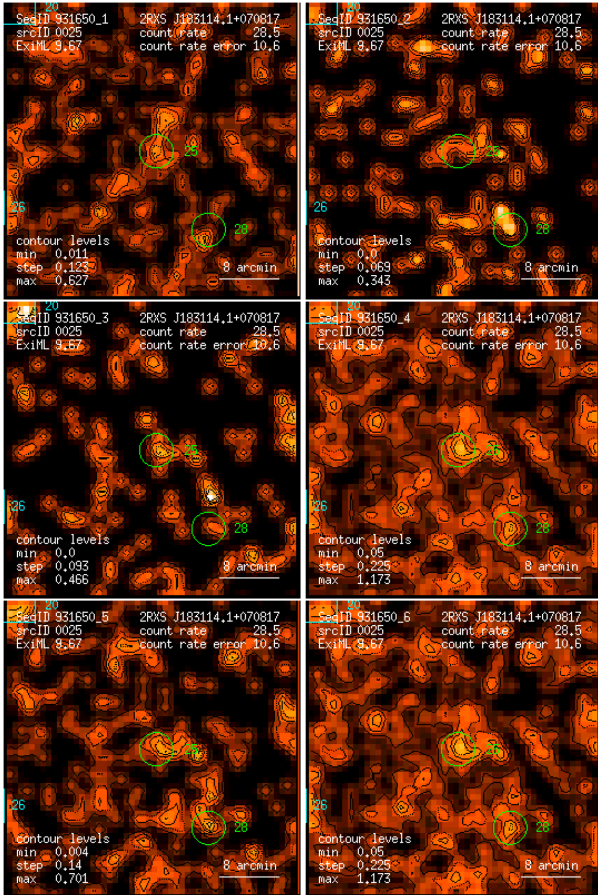
Figure 25: RASS 931650: detection 0025: band rate images, Gaussian filter: (1) PSPC channels 11 – 41, (2) 52 – 90, (3) 91 – 201, (4) 11 – 235, (5) 52 – 201, (6) 11 – 201. Broad band rates in counts/ks. Band rate contour levels in counts/ks/arcmin 2 .
