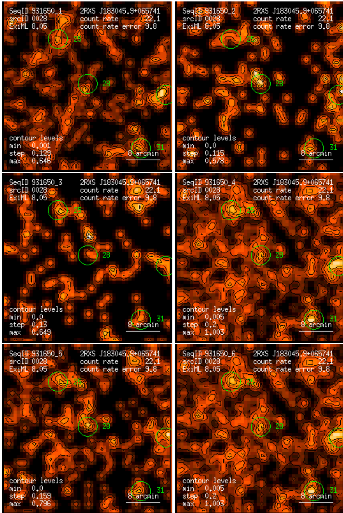
Figure 28: RASS 931650: detection 0028: band rate images, Gaussian filter: (1) PSPC channels 11 – 41, (2) 52 – 90, (3) 91 – 201, (4) 11 – 235, (5) 52 – 201, (6) 11 – 201. Broad band rates in counts/ks. Band rate contour levels in counts/ks/arcmin 2 .
