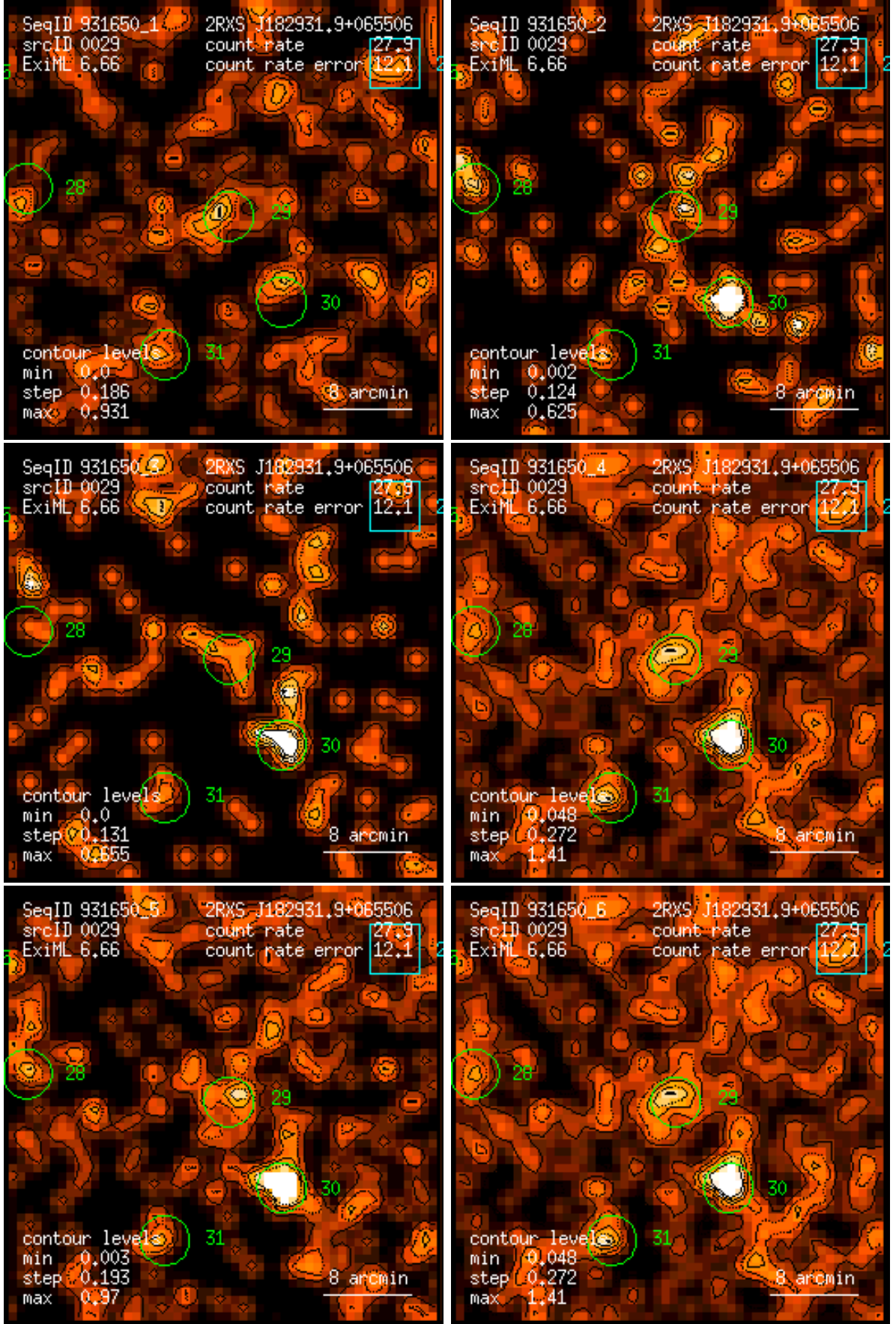
Figure 29: RASS 931650: detection 0029: band rate images, Gaussian filter: (1) PSPC channels 11 – 41, (2) 52 – 90, (3) 91 – 201, (4) 11 – 235, (5) 52 – 201, (6) 11 – 201. Broad band rates in counts/ks. Band rate contour levels in counts/ks/arcmin 2 .
