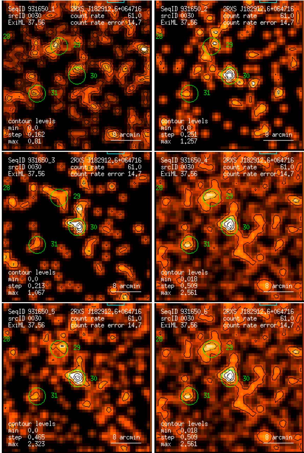
Figure 30: RASS 931650: detection 0030: band rate images, Gaussian filter: (1) PSPC channels 11 – 41, (2) 52 – 90, (3) 91 – 201, (4) 11 – 235, (5) 52 – 201, (6) 11 – 201. Broad band rates in counts/ks. Band rate contour levels in counts/ks/arcmin 2 .
