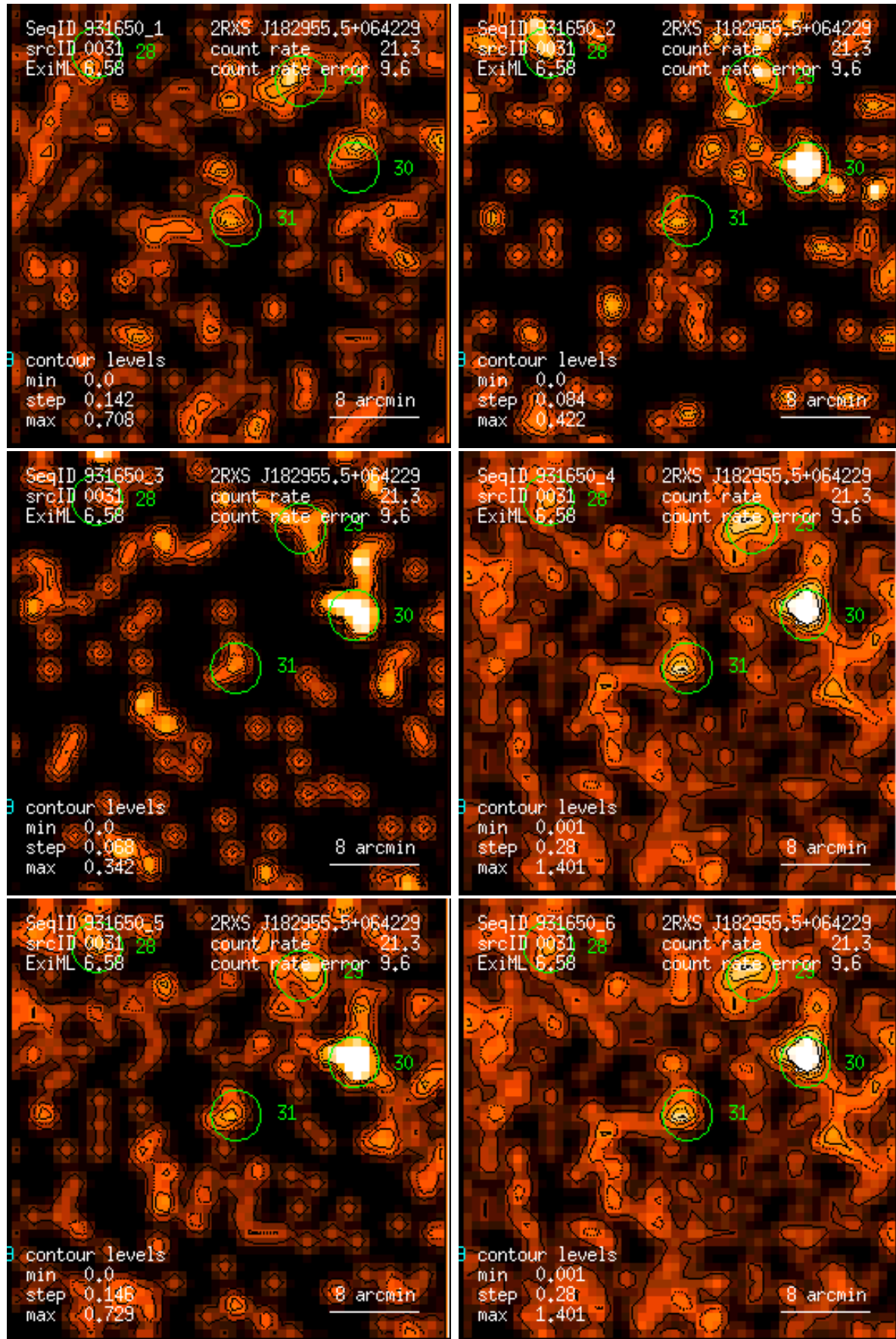
Figure 31: RASS 931650: detection 0031: band rate images, Gaussian filter: (1) PSPC channels 11 – 41, (2) 52 – 90, (3) 91 – 201, (4) 11 – 235, (5) 52 – 201, (6) 11 – 201. Broad band rates in counts/ks. Band rate contour levels in counts/ks/arcmin 2 .
