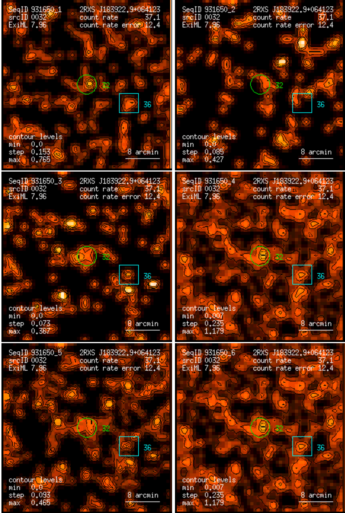
Figure 32: RASS 931650: detection 0032: band rate images, Gaussian filter: (1) PSPC channels 11 – 41, (2) 52 – 90, (3) 91 – 201, (4) 11 – 235, (5) 52 – 201, (6) 11 – 201. Broad band rates in counts/ks. Band rate contour levels in counts/ks/arcmin 2 .
